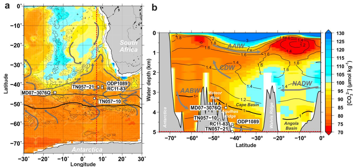
Figure 1. Location of the study cores. (a) Carbonate ion concentrations ( [CO_3^{2-}] ) in bottom waters in the Southeast Atlantic (Key et al., 2004), thin line tracks the 4- (stippled) and 2-km isobaths (solid); the position of major fronts are shown in dark gray (Polar Front), in gray (Sub-Antarctic Front), and in light gray (Sub-Tropical Front; Orsi et al., 1995; Sokolov & Rintoul, 2009); deep ocean currents are shown after Tucholke and Embley (1984) and Stramma and England (1999). (b) Meridional transect of [CO_3^{2-}] (shaded) and calcite saturation \Omega = [CO_3^{2-}]_{\text{in-situ}}/[CO_3^{2-}]_{\text{saturated}} (contoured) along 7°E (Key et al., 2004). Circles indicate the location of the study cores from the Cape Basin, and square shows sediment core used for comparison (Table S1). Deep water masses are indicated according to Talley (2013); AABW: Antarctic Bottom Water, NADW: North Atlantic Deep Water, CDW: Circumpolar Deep Water, AAIW: Antarctic Intermediate Water).
