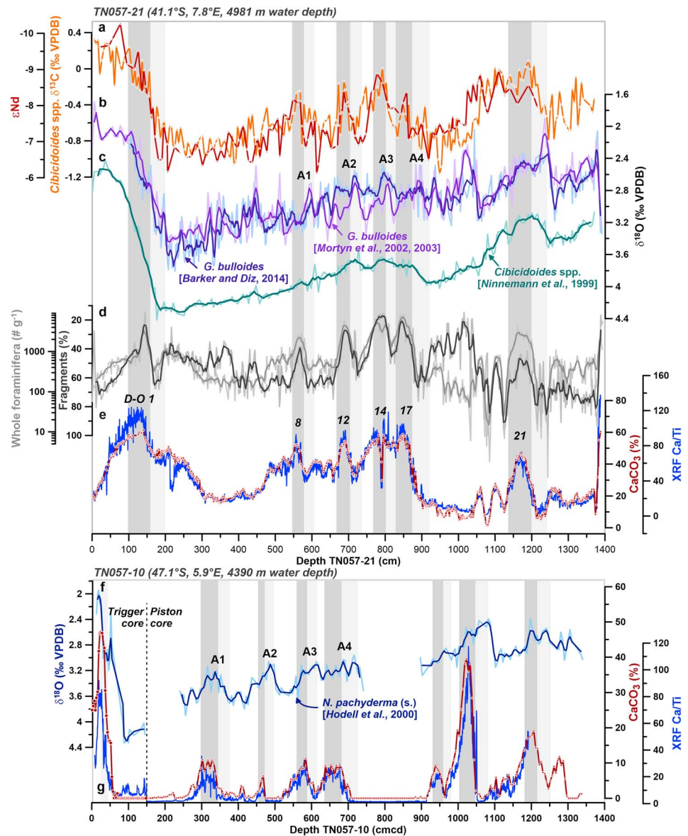
Figure 3. Millennial-scale changes in the carbonate chemistry of the deep Cape Basin during the last glacial cycle recorded in (top) TN057-21 and (bottom) TN057-10. (a) Cibicides spp. \delta^{13}\text{C} (orange; Ninnemann et al., 1999) and water mass source indicator \epsilon_{\text{Nd}} (dark red; Piotrowski et al., 2008, 2012), (b) G. bulloides \delta^{18}\text{O} data of Mortyn et al. (2002, 2003; purple) and Barker and Diz (2014; blue, depth scale adjusted), (c) Cibicides spp. \delta^{18}\text{O} (light green; Ninnemann et al., 1999), (d) number of whole planktic foraminifera per gram sediment (light gray; Barker & Diz, 2014) and planktic foraminifer fragmentation (dark gray), (e) coulometrically determined carbonate content (red, depth scale adjusted; Sachs & Anderson, 2003) and the XRF Ca/Ti ratio (blue), (f) N. pachyderma (s.) \delta^{18}\text{O} (Hodell et al., 2000), and (g) coulometrically determined carbonate content (red; Channell et al., 2000; Kanfoush et al., 2000) and the XRF Ca/Ti ratio (blue). Light gray bars highlight decreases and/or minima in planktic \delta^{18}\text{O} , that is, phases of surface warming that have likely paralleled Antarctic warming events (A1-A4; numbering after Blunier & Brook, 2001). Dark gray bars highlight intervals of pronounced carbonate preservation that coincide with strong and prolonged Dansgaard-Oeschger (D-O, numbering after Dansgaard et al., 1993) interstadials.
