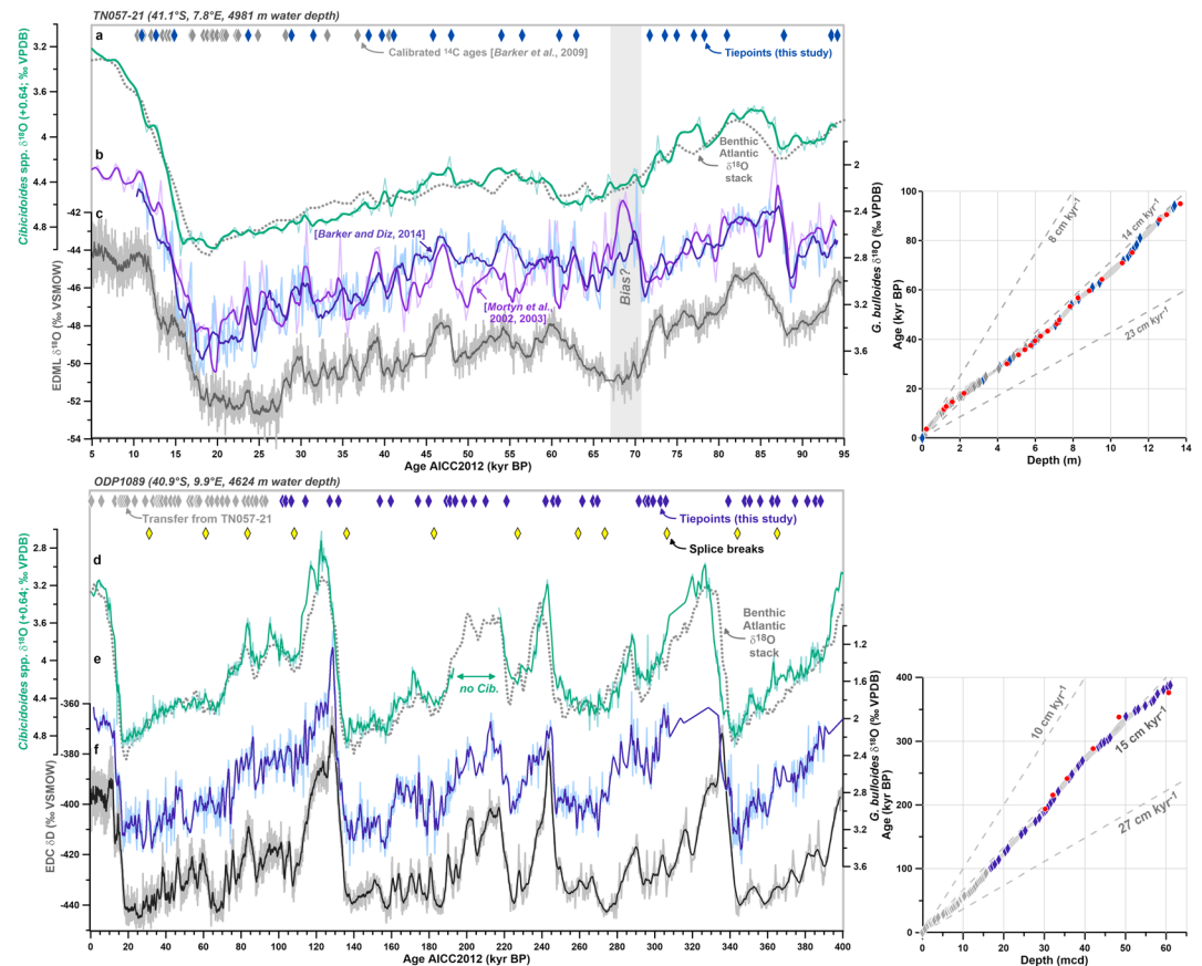
Figure 4. Age model (top) for sediment core TN057-21 and (bottom) for ODP Site 1089. (a) Cibicides spp. \delta^{18}\text{O} (green; Ninnemann et al., 1999) and the Atlantic benthic \delta^{18}\text{O} stack of Lisiecki and Raymo (2009; stippled), (b) G. bulloides \delta^{18}\text{O} data of Mortyn et al. (2002, 2003; purple) and Barker and Diz (2014; blue, depth scale adjusted), (c) \delta^{18}\text{O} of the Antarctic EPICA Dronning Maud Land (EDML) ice core (gray; EPICA Community Members, 2006), (d) Cibicides spp. \delta^{18}\text{O} (green; Hodell et al., 2001) and the Atlantic benthic \delta^{18}\text{O} stack of Lisiecki and Raymo (2009) (stippled), (e) G. bulloides \delta^{18}\text{O} (Mortyn et al., 2002, 2003), and (f) EPICA Dome C (EDC) \delta\text{D} (Jouzel et al., 2007). Symbols at the top of each panel indicate age markers (TN057-21: ^{14}\text{C} dating [gray] and stratigraphic alignment of G. bulloides \delta^{18}\text{O} to Antarctic temperature [blue]; ODP Site 1089: tie points transferred from TN057-21 [gray] and from a stratigraphic alignment of G. bulloides \delta^{18}\text{O} and Antarctic temperature variations [blue], and splice breaks [yellow]). Insets on the right show age–depth relationships for the core sites in comparison to previous chronologies (red) for TN057-21 (Barker & Diz, 2014) and for ODP Site 1089 (Stoner et al., 2003), age uncertainties (gray envelopes) and sedimentation rates (stippled lines). Gray bar in the top panel indicates a potential bias of G. bulloides \delta^{18}\text{O} owing to seasonality or dissolution (Barker & Diz, 2014).
