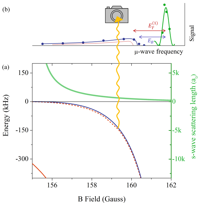
FIG. 1. (a) The solid green line shows the two-body scattering length near the Feshbach resonance centered at 155.04 G. The solid red line is the calculated energy of the ground state Efimov trimer, E_T^{(0)} [22]. The solid blue and dashed red lines show the calculated molecular energies of the Feshbach dimer, E_b , and first excited Efimov trimer, E_T^{(1)} , respectively. We populate molecular states by sweeping our gas from 155.04 G to B > 158.6 G. With a microwave pulse, we then transfer either atomic or molecular population to the |3, -3\rangle state for absorption imaging; the experimental points in (b) are population transfer. The green line is a delta function free-atom transition broadened by experimental resolution. The blue line is a calculated Frank-Condon factor for dimer dissociation [23]. The red line shows the expected shape of the trimer dissociation yield, but the difference between E_T^{(1)} and E_b is exaggerated for clarity.
