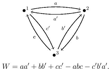
FIGURE 38. The quiver with potential for the 3-punctured sphere.
