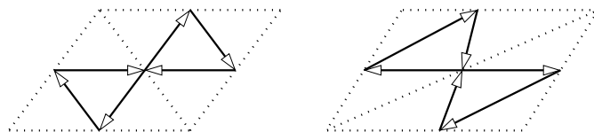
FIGURE 2. Effect of a flip.
