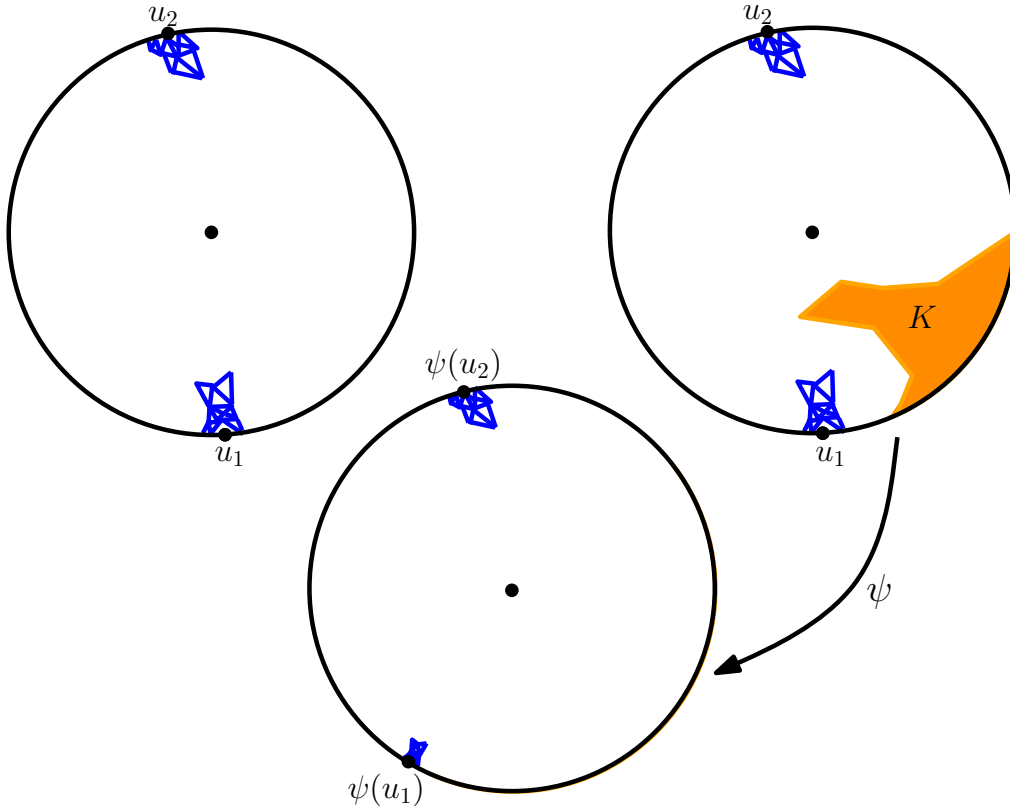
Figure 1.4: Upper left: Suppose a discrete random triangulation is conformally mapped to the disk, and the Eden model growing from the boundary inward takes about N time units to absorb the cluster of triangles shown near u_1 , and also about N units to absorb the cluster near u_2 . (Other not-shown triangles scattered around the boundary are also added during that time.) Upper right: Now suppose that we modify the initial setup by designating the hull K to be part of the boundary. Intuitively, if the regions near u_1 and u_2 are small, this modification should not affect the relative rate at which growth happens near u_1 and u_2 . That is, there should be some N' such that both clusters take about N' steps to be absorbed. Bottom: A conformal map \psi: \mathbf{D} \setminus K \rightarrow \mathbf{D} with \psi(0) = 0 scales the region near u_i by about |\psi'(u_i)| . The capacity corresponding to the shown blue cluster near \psi(u_i) is approximately |\psi'(u_i)|^2 times that of the original blue cluster near u_i . This suggests that if (\nu_t) is the driving measure in the bottom figure and (\tilde{\nu}_t) is the original driving measure in the upper left, and I_i is a small interval about u_i , then \nu_0(\psi(I_i)) should be roughly proportional to |\psi'(u_i)|^2 \tilde{\nu}_0(I_i) . In the \eta -DBM model, one replaces |\psi'(u_i)|^2 by |\psi'(u_i)|^{2+\eta} because the rate at which particles reach u_i should also change by a factor roughly proportional to |\psi'(u_i)|^\eta .
