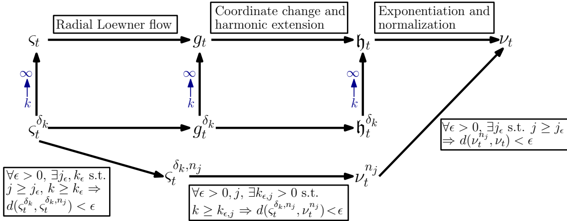
Figure 6.3: (Continuation of Figure 6.2.) Shown is the approximation scheme used to show that \varsigma_t = \nu_t (Proposition 6.12) to complete the proof of the existence of \text{QLE}(\gamma^2, \eta) for (\gamma^2, \eta) on one of the upper two curves from Figure 1.3. The statements in each of the three boxes along the bottom of the figure from left to right are proved in Lemma 6.13, Lemma 6.14, and Proposition 6.11, respectively. The symbol d represents a notion of “closeness” which is related to the topology of \mathcal{N} . To show that \varsigma_t = \nu_t , we first pick j very large so that d(\nu_t^{n_j}, \nu_t) < \epsilon and d(\varsigma_t^{\delta_k}, \varsigma_t^{\delta_k, n_j}) < \epsilon . We then pick k very large so that d(\varsigma_t^{\delta_k}, \varsigma_t) < \epsilon and d(\varsigma_t^{\delta_k, n_j}, \nu_t^{n_j}) < \epsilon .
