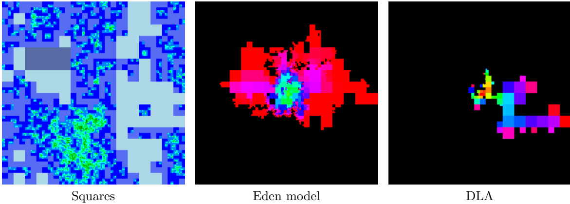
Figure 1.13: \gamma = 2
