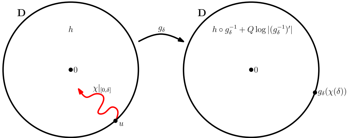
Figure 6.1: Fix \kappa > 1 and suppose that (h, u) has the law as described in Proposition 4.7 (where the role of \gamma in the application of the proposition is played by 2\alpha_\kappa ) plus -\frac{\kappa+6}{2\sqrt{\kappa}} \log |\cdot| and let \nu_{h,\kappa} be the -\frac{2}{\sqrt{\kappa}} -quantum boundary length measure associated with h . Then the conditional law of h given u is that of a free boundary GFF on \mathbf{D} plus -\frac{\kappa+6}{2\sqrt{\kappa}} \log |\cdot| + \frac{2}{\sqrt{\kappa}} \log |\cdot - u| . By Theorem 5.1, the law of the pair (h, u) is invariant under the operation of sampling a radial \text{SLE}_\kappa process in \mathbf{D} starting from u and targeted at 0 (which given u is conditionally independent of h ) up to some fixed (log conformal radius) time \delta , mapping back using the (forward) radial Loewner map g_\delta as illustrated above, and applying the change of coordinates formula for quantum surfaces. Here, h is viewed as a modulo additive constant distribution. This is the basic operation which is used to construct QLE.
