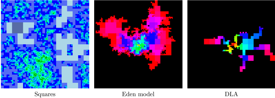
Figure 1.12: \gamma = 7/4
