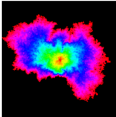
Eden model
