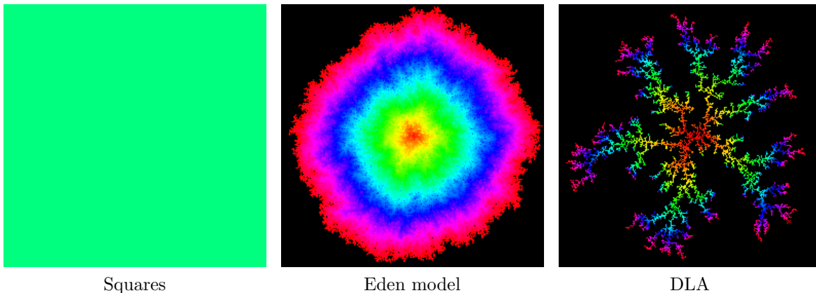
Figure 1.5: \gamma = 0
