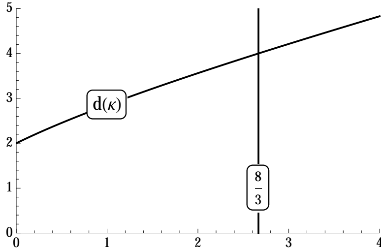
Figure 3.1: The value d as a function of \kappa = \gamma^2 , as defined by (3.6). Although the graph is not a straight line, it appears “almost straight” and it takes the value 2 for \kappa = 0 and 4 for \kappa = 8/3 .
