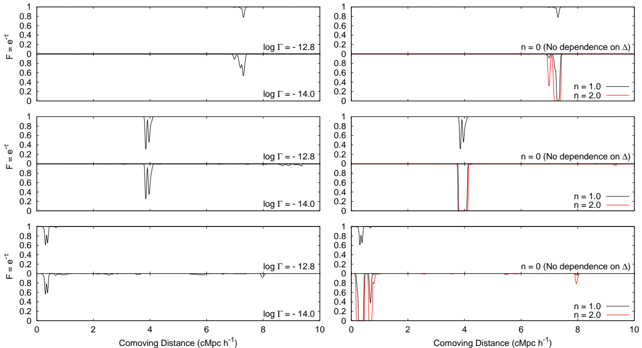
Figure 3. Left: Comparison of simulated O I spectra for two different background photo-ionization rates for three different sightlines through the simulation at z = 6.0 . The Rahmati et al. (2013a) self-shielding model was used. The top spectrum has \log(\Gamma/\text{s}^{-1}) = -12.8 and the bottom spectrum has \log(\Gamma/\text{s}^{-1}) = -14.0 . The metallicity is Z = 10^{-2} Z_{\odot} . Right: Comparison of simulated O I spectra for different values of the power law index n of the metallicity model. The Rahmati et al. (2013a) self-shielding model was used with background photo-ionization rate \log(\Gamma/\text{s}^{-1}) = -12.8 .
