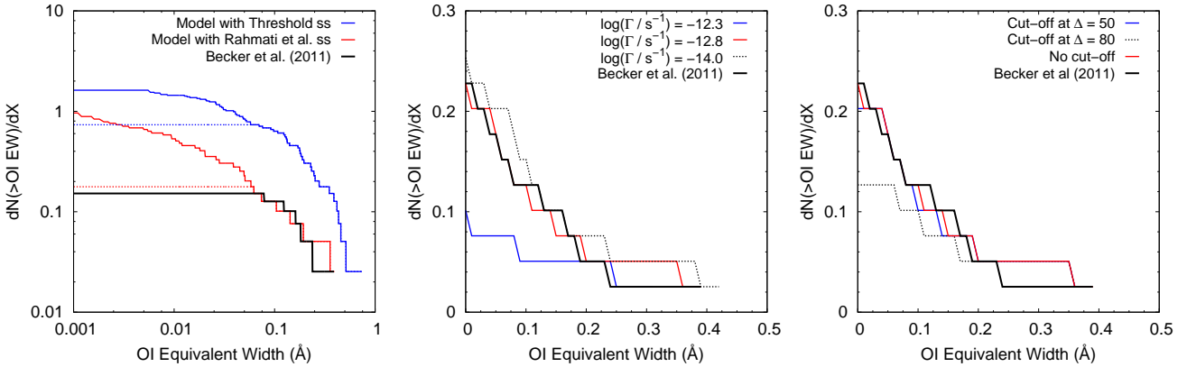
Figure 5. The cumulative incidence rate of simulated O I absorbers compared to the observed distribution obtained by Becker et al. (2011). The left panel is for the metallicity model that fits the data with the Rahmati et al. (2013a) self shielding model ( Z = 10^{-2.65} Z_{\odot} (\Delta/80)^{1.3} ). The dashed/solid curves are with/without the Becker et al. completeness correction. The middle panel shows the cumulative incidence rate of simulated O I absorbers assuming different background photo-ionization rates \Gamma and the Rahmati et al. (2013a) self-shielding model. The completeness correction shown in the right panel of Fig. 4 has been applied to the curves. The metallicity model used is the same as in the left panel. The right panel shows the effect of introducing different cut-off overdensities, below which the metallicity is set to zero. The red curve assumes a power law model for the metallicity that extends to arbitrarily low density. The blue curve assumes that regions with \Delta < 50 contain no metals. The black dashed curve assumes that there are no metals below a cut-off overdensity of \Delta = 80 . The thick black curve shows the observed cumulative incidence rate of O I absorbers obtained by Becker et al. (2011). The metallicity model used is the same as in the left panel.
