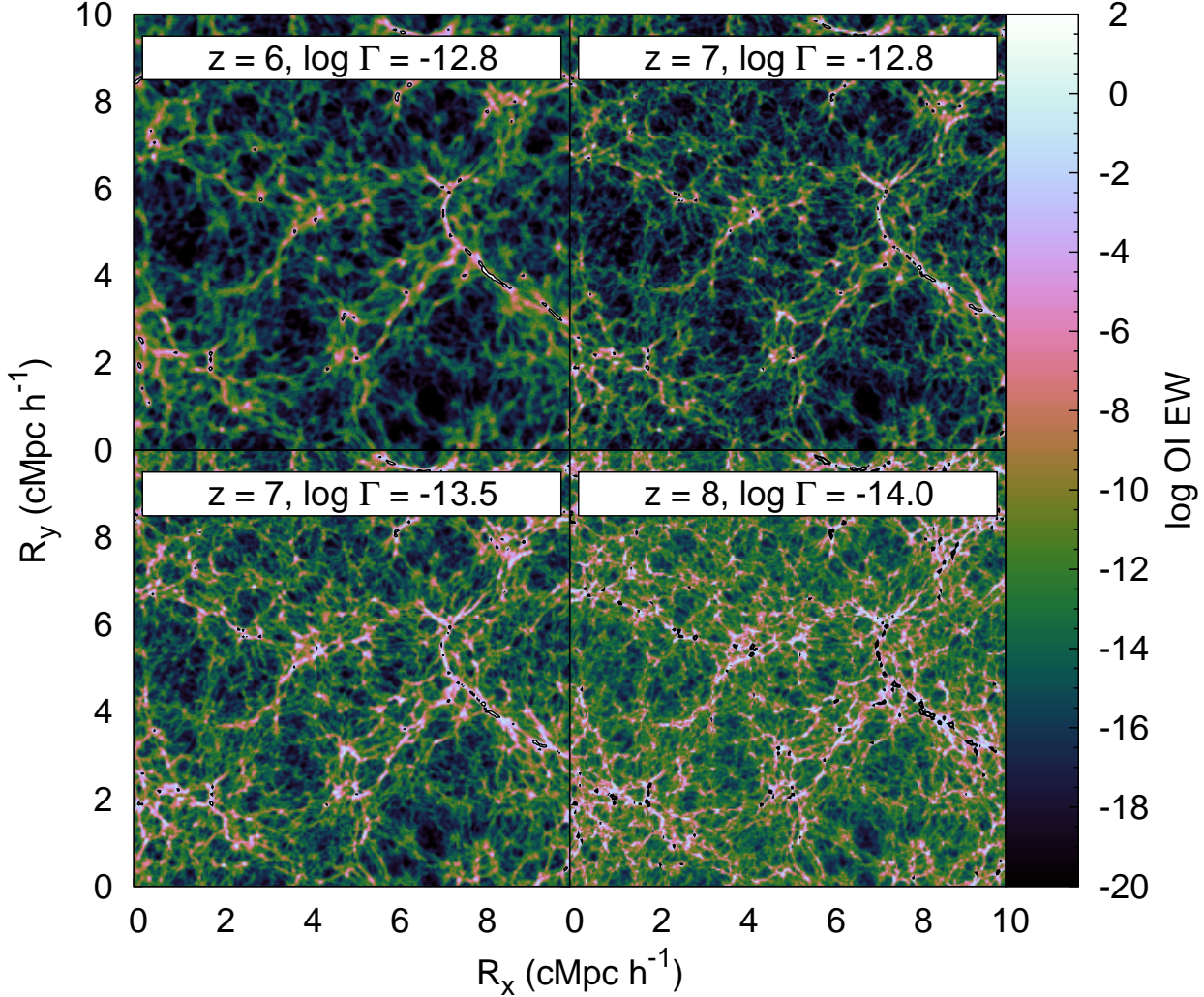
Figure 8. The location of O I absorbers in the simulation. The O I equivalent width was estimated from the H I column density (see Figure 4). The H I column density was calculated by integrating n_{\text{HI}} over the thickness ( 39h^{-1} ckpc) of the slice shown in the plot. The distribution of O I absorbers is shown for \log \Gamma = -12.8 at z = (6.0, 7.1) , for \log \Gamma = -13.5 at z = 7.1 and for \log \Gamma = -14.0 at z = 8.0 . The Rahmati et al. (2013a) model for self-shielding was used in each case. The black contours enclose absorbers with \text{EW}_{\text{OI}} \geq 0.01 \text{ \AA} .
