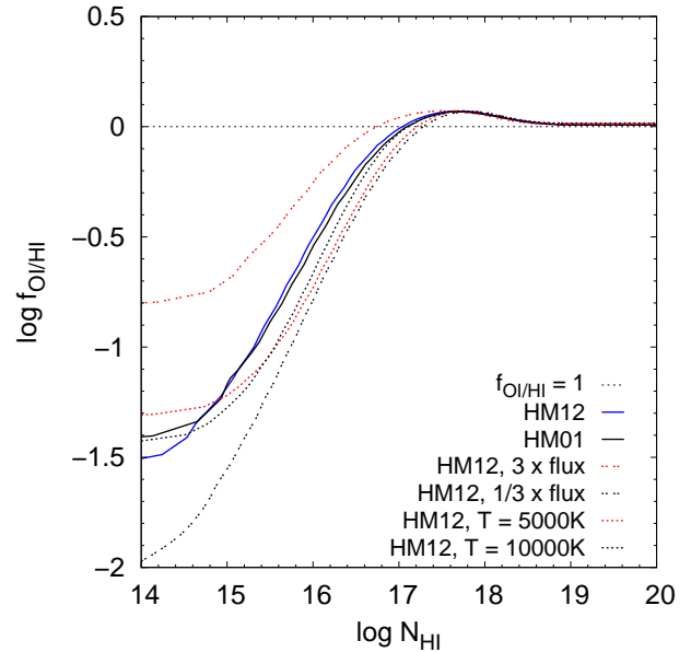
Figure A1. Plot of the neutral fraction of oxygen relative to the neutral fraction of hydrogen against H I column density. The blue curve assumes the Haardt & Madau (2012) UV background model. We find that O I is a good tracer of H I for self-shielded gas with \log N_{\text{HI}} \gtrsim 17 . Calculations for the Haardt & Madau (2001) model of the UV background and for decreased/increased amplitude of the UV background and constant temperature of the gas of 5000K and 10000K are also shown. The dashed line shows f_{\text{OI}/\text{HI}} = 1 .
