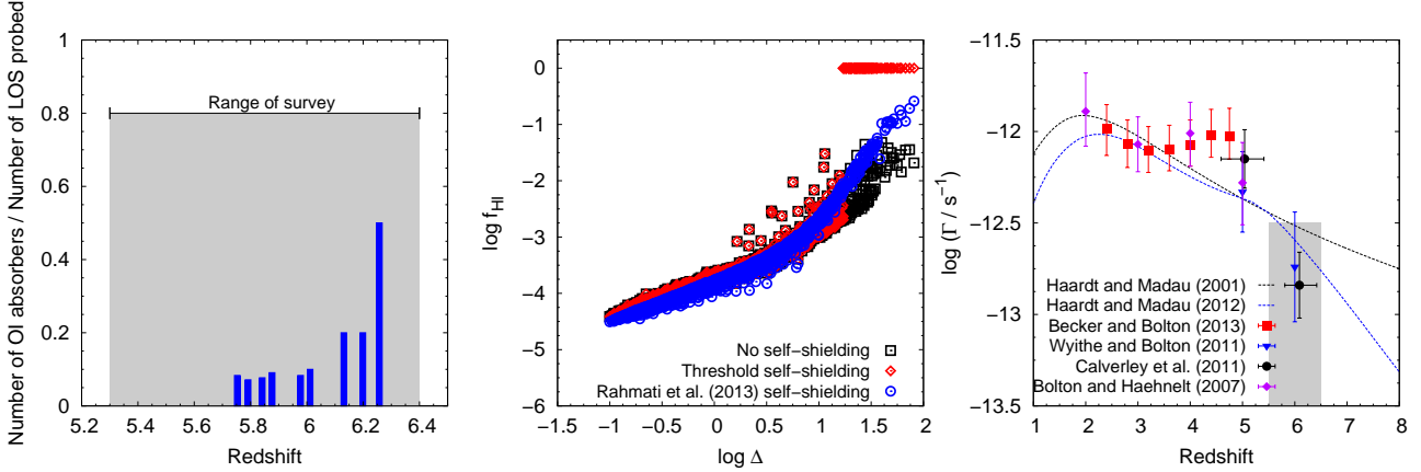
Figure 1. Left: The incidence rate of O I absorbers in the survey of Becker et al. (2011). Nine systems containing O I were detected. The height of the bars is the ratio of the number of O I absorbers to the number of sightlines that were surveyed at the redshift of the absorber. All of the O I absorption systems were found at z > 5.75 and the line of sight number density of absorbers appears to increase rapidly with increasing redshift. Middle: The dependence of neutral fraction on overdensity for the simulation with no self-shielding, with the threshold self-shielding model used in Bolton & Haehnelt (2013) and the self-shielding prescription used in Rahmati et al. (2013a). The photo-ionization rate in this case was taken to be \log(\Gamma/\text{s}^{-1}) = -12.8 . Right: A plot of the background photo-ionization rate \Gamma against redshift z . The points are measurements of the UV background at different redshifts taken from Becker & Bolton (2013), Wytthe & Bolton (2011), Calverley et al. (2011) and Bolton & Haehnelt (2007). The Haardt & Madau (2001) and Haardt & Madau (2012) models for \Gamma are also shown. The shaded grey region shows the range of \Gamma consistent with the observed incidence rate of O I absorbers at z \sim 6 .
