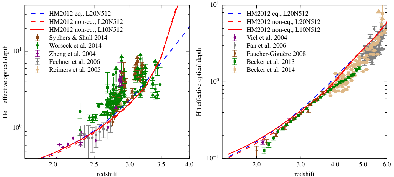
Figure 5. Effective optical depths for He II ( left panel ) and H I ( right panel ) Lyman- \alpha absorption as a function of redshift. The results are based on equilibrium and non-equilibrium simulations with the HM2012 UV background. Observational constraints on the He II effective optical depth from Zheng et al. (2004), Reimers et al. (2005), Fechner et al. (2006), Syphers & Shull (2014) and Worseck et al. (2014) are shown for reference. For the H I effective optical depth, we compare to data from Viel et al. (2004), Fan et al. (2006), Faucher-Giguère et al. (2008a), Becker et al. (2013) and Becker et al. (2014). The x-axis is linear in \log(1+z) so that a power-law evolution corresponds to a straight line.
