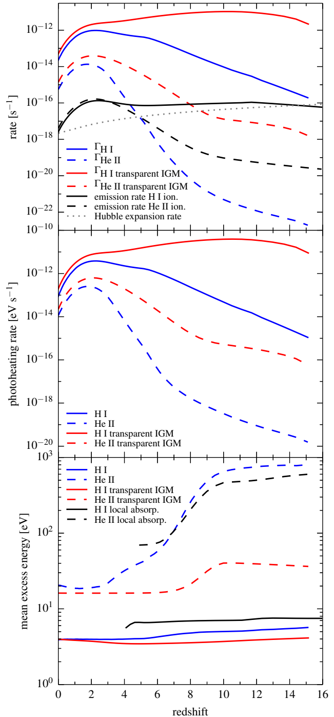
Figure 1. Top panel: Ionizing photon emission and photoionization rates for hydrogen and singly-ionized helium in the HM2012 model. For comparison, the photoionization rates are also shown in the transparent IGM limit. The emission rates of H I and He II ionizing radiation are plotted per hydrogen and helium atom (including all ionization states), respectively. The Hubble expansion rate H(z) is also indicated. Middle panel: Photoheating rates for H I and He II as a function of redshift in the HM2012 model as well as in the transparent IGM limit. Lower panel: Mean excess energy per H I and He II ionization in the HM2012 model, as well as in the transparent IGM and immediate local absorption limits.
