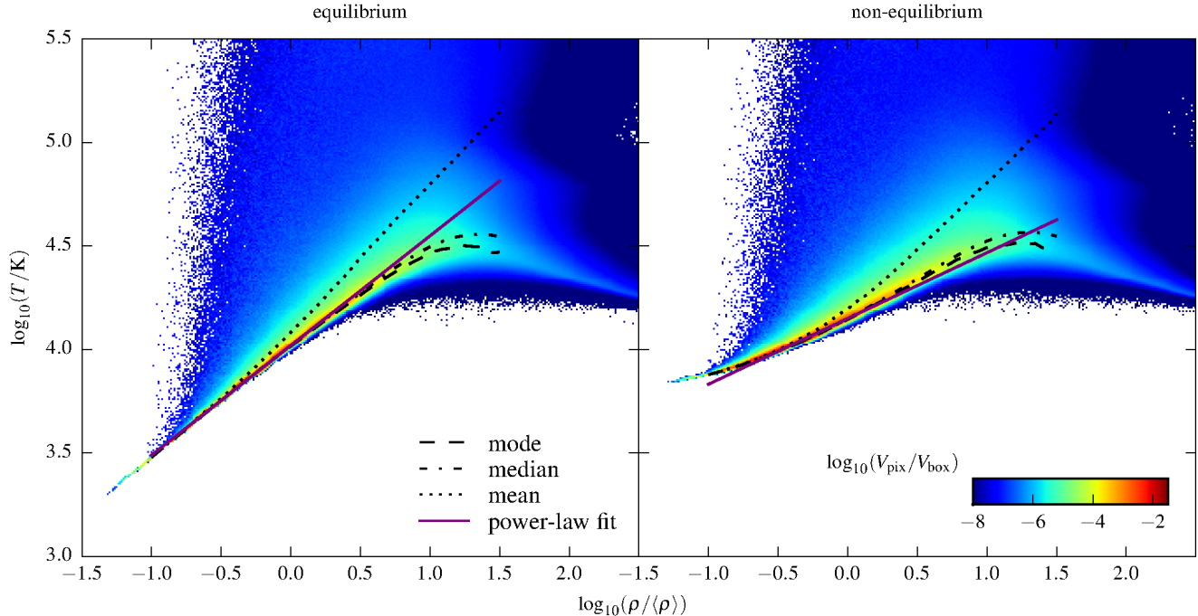
Figure 2. The volume-weighted distribution of gas in the temperature-density plane in equilibrium ( left panel , run L20N512 HM2012 eq.) and non-equilibrium ( right panel , run L20N512 HM2012 non-eq.) simulations with a HM2012 UVB. The results are given at z = 3.5 , i.e. shortly after the bulk of the He II has been reionized in these models.
