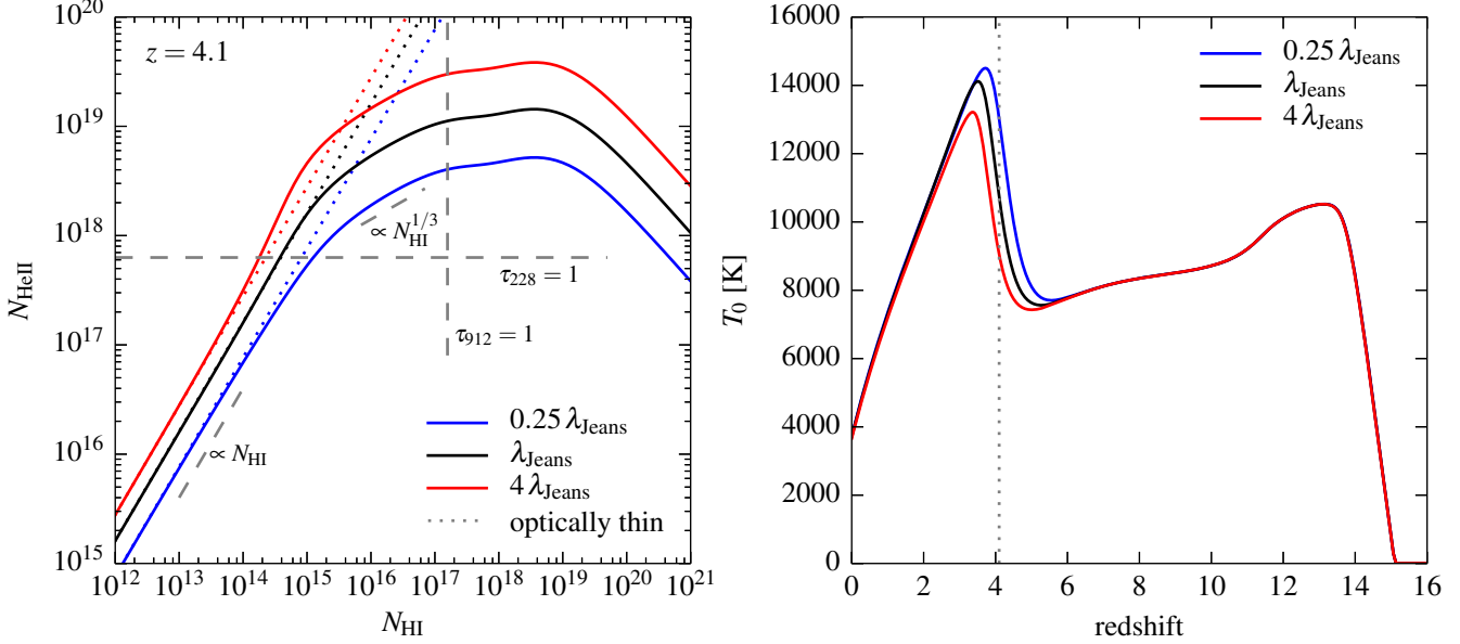
Figure C1. The left panel illustrates the conversion from the H I to the He II column density of an absorber in the HM2012 model. In particular it shows how the conversion depends on the assumed size of the absorber in units of the Jeans length. Results are shown for absorber sizes of 0.25, 1 and 4 times the Jeans length at z = 4.1 . The right panel shows how the evolution of the IGM temperature at mean density depends on the assumed absorber size. The curves are based on a non-equilibrium treatment of photoheating.
