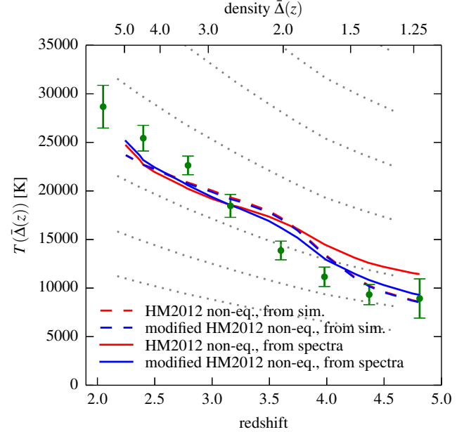
Figure 6. Comparison of IGM temperatures computed directly from the simulations ( dashed , indicating T_{\text{power law}} in the L10N512 runs) and obtained from the curvature of synthetic Lyman- \alpha forest spectra ( solid ). The temperatures are shown at the densities \bar{\Delta}(z) to which the curvature method is most sensitive. Results for a non-equilibrium simulation with the HM2012 UVB are shown by red lines. The blue lines indicate results for a non-equilibrium run with the modified HM2012 background in which H I and He I reionization happen later. The Becker et al. (2011) observational constraints ( green circles and error bars ) are shown for reference. The temperatures in the reference simulations, which these authors used to calibrate a curvature-temperature relation, are indicated by the grey dotted lines.
