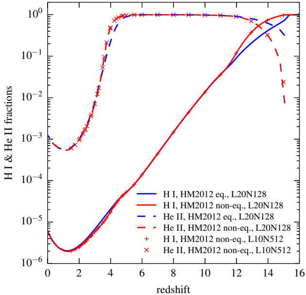
Figure A1. Ionization fractions as a function of redshift for simulations with equilibrium and non-equilibrium photoheating. The results are based on the HM2012 UVB. Shown are the ratios of the number of H I to the number of all hydrogen atoms and of the number of He II to all helium atoms. The L20N512 simulation is in excellent agreement with the other runs and not shown for clarity.
