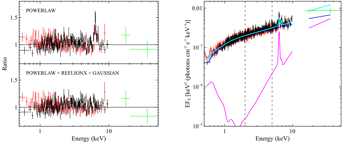
FIG. 1.— Left : data/model ratios for a simple absorbed powerlaw, and a powerlaw with a distant reflector and a Gaussian emission line. Right : the relative contributions of the powerlaw (blue) and distant reflection (magenta), the latter indicating the upper limit obtained for the reflection in the marked 2–5 keV bandpass. XIS FI, BI and PIN data are shown in black, red and green, and the total model in cyan; spectra have been rebinned and the additional Gaussian omitted from display for visual clarity. The broadband spectrum is dominated by the intrinsic powerlaw continuum.
