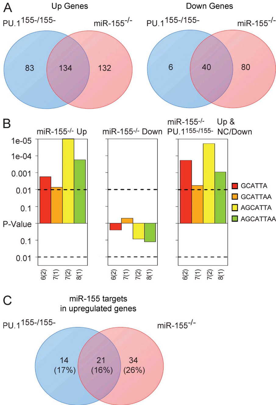
Figure 7. PU.1 explains a large fraction of changes in the transcriptome of miR-155-deficient B cells. (A) Venn diagrams representing the number of genes up-regulated or down-regulated in PU.1 155-/-/155- , or miR-155 -/- samples, compared with WT. All genes tested are from the DEG group of genes listed in Table S1. (B) Sylamer analysis for genes either up- or down-regulated in miR-155 -/- compared with WT, for enrichment of miR-155-binding sites (6-mer, 7-mer, or 8-mer composition). Also tested were genes up-regulated in miR-155 -/- but down-regulated or without change in expression in PU.1 155-/-/155- samples. Significance was calculated by comparing enrichment of the miR-155 seed sequence in these selected groups of genes to all the genes containing a 3'UTR in the mouse genome. (C) Venn diagram intersecting the number of genes with miR-155-binding sites in PU.1 155-/-/155- or miR-155 -/- up-regulated genes. Percentages in brackets represent the number of genes with miR-155-binding sites as a proportion of the total number of up-regulated genes.
