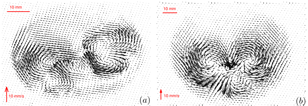
FIGURE 16. Average velocity fields at late times for fractures in the toughness regime. (a) t/t_{mk} \sim 10^{12} (piv1) and (b) t/t_{mk} \sim 10^{11} (piv2).
