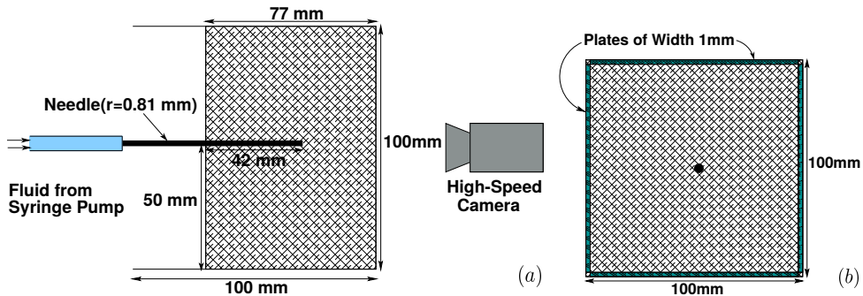
FIGURE 2. Schematic diagrams of the experimental setup. (a) Elevation view and (b) plan view.
