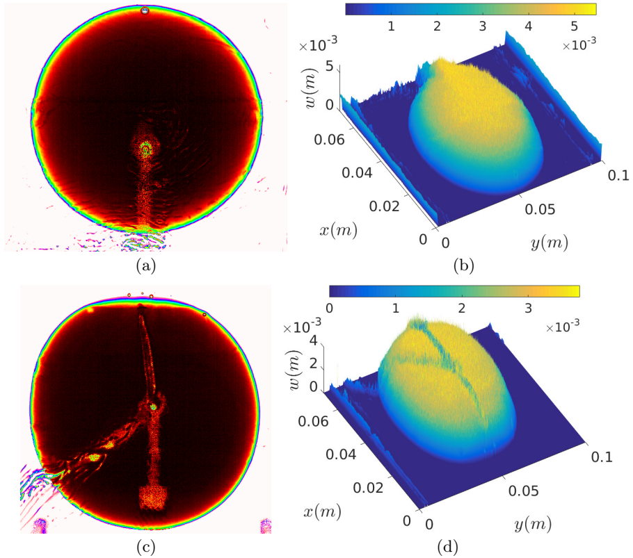
FIGURE 4. Experimental radial and aperture profiles of sample experiments. 4(a) & 4(b) exp8 ( t \approx 39.4 s). 4(c) & 4(d) exp15 ( t \approx 40.6 s).
