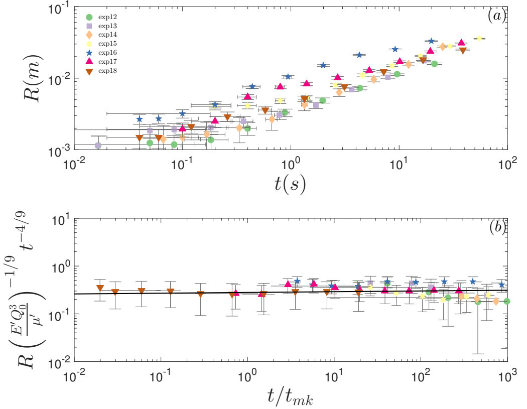
FIGURE 7. (a) The growing crack radius R versus time for a number of experiments with varying injection rate Q , viscosity \mu and elastic modulus E . (b) The viscosity rescaling R_m(t) of crack dependence versus rescaled time t/t_{mk} .
