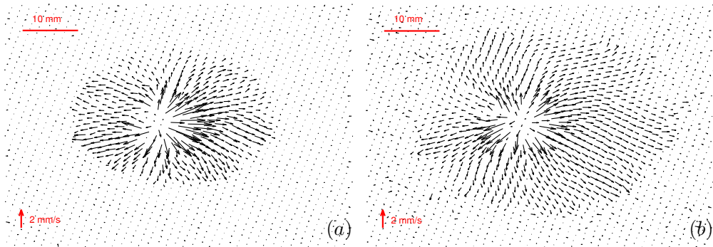
FIGURE 13. Velocity fields for a fractures in the viscosity regime (piv4). (a) t/t_{mk} \sim 10 and (b) t/t_{mk} \sim 20 .
