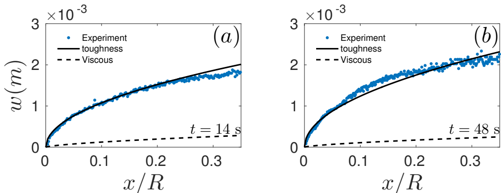
FIGURE 11. The crack tip region for a toughness dominated fracture (exp10) which follows the LEFM toughness asymptote (2.41) denoted by the solid line. (a) t/t_{mk} = 1.4 \times 10^8 and (b) t/t_{mk} = 4.8 \times 10^8 .
