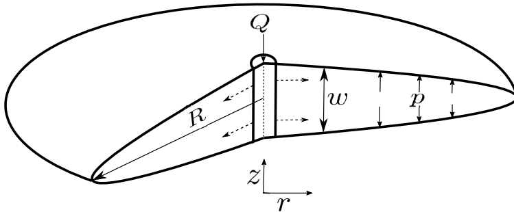
FIGURE 1. Schematic diagram showing the radial fracture geometry.
