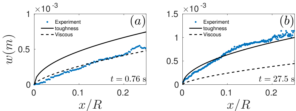
FIGURE 12. The crack tip region for a fracture (exp16) which transitions from the viscous dissipation (2.42) to the toughness asymptote (2.41), denoted by the dashed and solid lines respectively. (a) t/t_{mk} = 76 and (b) t/t_{mk} = 2.8 \times 10^3 .
