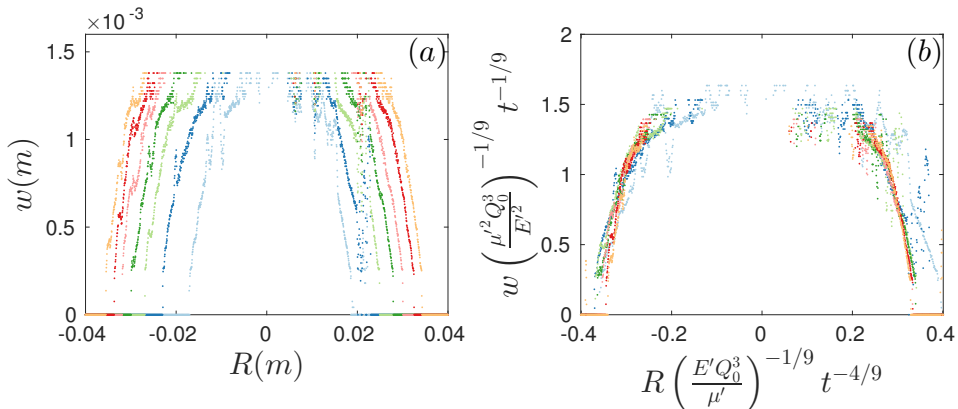
FIGURE 10. (a) The crack aperture profile of a cross section, intersecting the injection needle, of the radial fracture for experiment exp16 (table 2), with \Delta t = 4 s. (b) The rescaled fracture aperture profile using the viscosity dominated radial and width power-law scalings from table 1.
