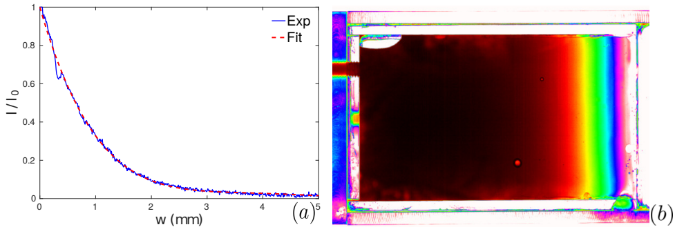
FIGURE 3. (a) The normalised light intensity I/I_0 versus the corresponding aperture of the fluid filled region for a given dye concentration. (b) Experimental image of a calibration using glycerin.
