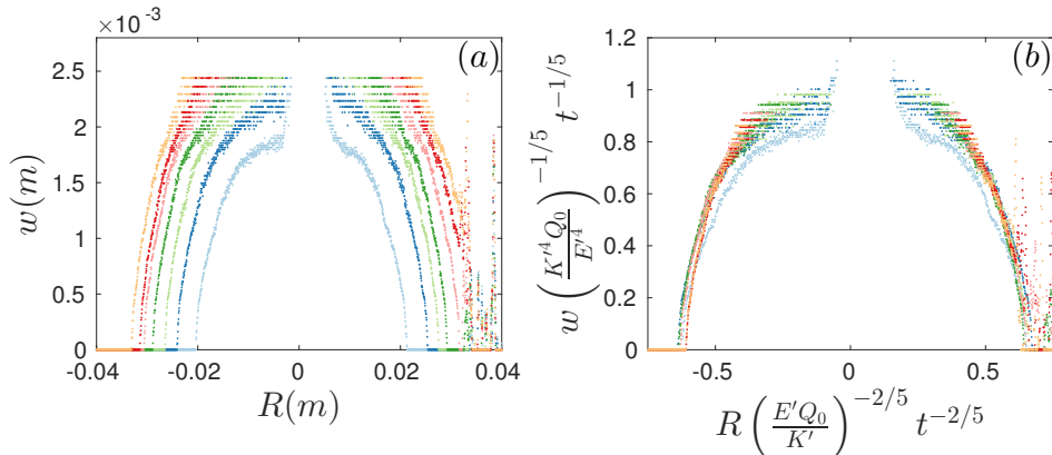
FIGURE 9. (a) The crack aperture profile of a cross section, intersecting the injection needle, of the radial fracture for experiment exp9 (table 2). Each set of data points corresponds to the crack aperture at a certain time, with time evolving outwards in increments of \Delta t = 4 s from the crack centre for each curve. (b) The rescaled fracture aperture profile using the toughness dominated radial and width power-law scalings from table 1.
