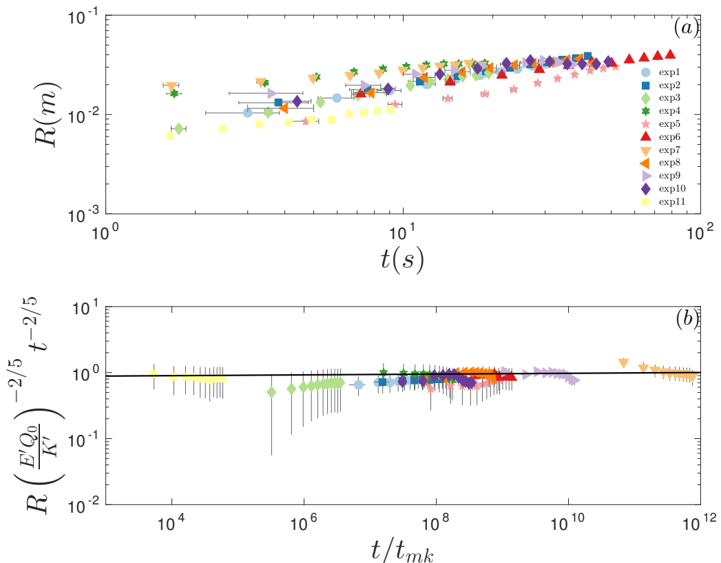
FIGURE 6. (a) The growing crack radius R versus time for a number of experiments with varying injection rate Q , viscosity \mu and elastic modulus E . (b) The toughness rescaling R_k(t) of crack dependence versus rescaled time t/t_{mk} .
