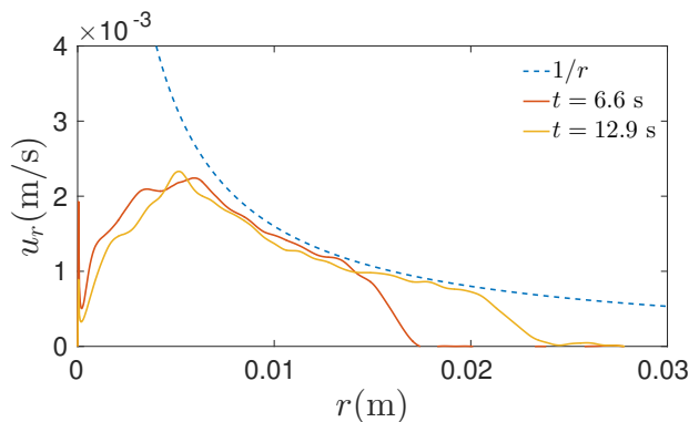
FIGURE 14. Azimuthal velocity average of fluid versus distance from the source r .
