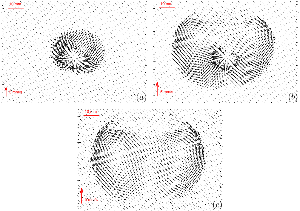
FIGURE 15. Average velocity fields at different stages for a fracture transitioning between regimes (piv3). (a) t/t_{mk} \sim 5 \times 10^2 , (b) t/t_{mk} \sim 5 \times 10^3 and (c) t/t_{mk} \sim 1 \times 10^4 .
