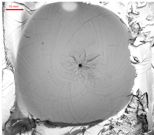
FIGURE 5. A typical fracture surface post experiment exhibiting spiral patterns (exp9).
