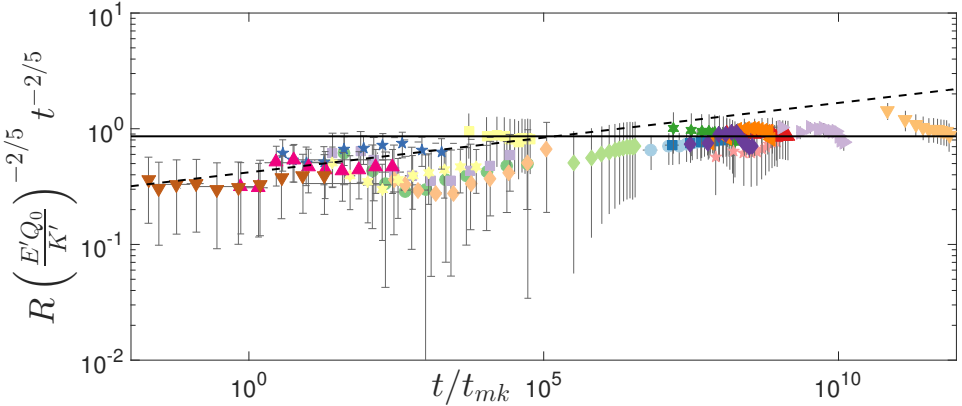
FIGURE 8. All experiments scaled using the radial toughness dominated power-law (2.31).
