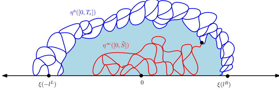
Figure 3: Illustration of the proof of Theorem 3.2. On the event F_\epsilon(l^L + l^R) , the auxiliary SLE 6 curve \eta^a (blue) forms a bubble D_\epsilon (light blue region) which disconnects 0 from \infty such that \partial D_\epsilon \cap \mathbb{R} is close to the interval [\xi(-l^L), \xi(l^R)] which has l^L units of \nu_{h^\infty} -length to the left of 0 and l^R units of \nu_{h^\infty} -length to the right of 0; and \nu_{h^\infty}(\partial D_\epsilon \setminus \mathbb{R}) is small. In the limit as \epsilon \rightarrow 0 , the quantum surface parameterized by D_\epsilon and the SLE 6 curve \eta^\infty (red), stopped at the first time \widehat{S} it hits \eta^a([0, T_\epsilon]) , converge in law to the curve-decorated quantum surface (\mathcal{B}, \eta_{\mathcal{B}}) appearing in Theorem 3.2 in a rather strong sense (Lemma 3.4). Since the left/right boundary length process Z^a for \eta^a evolves as a pair of independent 3/2-stable processes with no upward jumps, we can compute the probability of F_\epsilon(l^L + l^R) and the conditional probability of F_\epsilon(l^L + l^R) \cap \{\widehat{S} < u\} given the curve-decorated quantum surface (\mathcal{K}_u^\infty, \eta_{\mathcal{K}_u^\infty}) corresponding to an initial segment of \eta^\infty (Lemma 3.3). From these computations together with Bayes' rule, we obtain the Radon-Nikodym derivative of the conditional law of (\mathcal{K}_u^\infty, \eta_{\mathcal{K}_u^\infty}) given F_\epsilon(l^L + l^R) \cap \{\widehat{S} < u\} with respect to the marginal law of (\mathcal{K}_u^\infty, \eta_{\mathcal{K}_u^\infty}) (Lemma 3.7). Taking a limit as \epsilon \rightarrow 0 yields the theorem statement.
