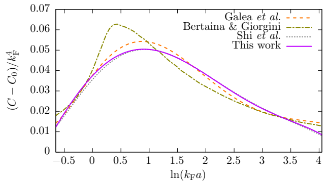
FIG. 5. (Color online) Contact minus the contact contribution from the molecular bound state, normalized by the fourth power of the Fermi wave vector. For comparison we also show the results from Refs. [21–23].
