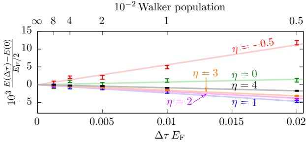
FIG. 11. (Color online) Variation of the dimensionless ground-state energy per particle with DMC time step and walker population with interaction parameter \eta = \ln(k_F a) in the zero-range limit k_F^2 R_{\text{eff}}^2 = 0 . The straight lines show a weighted least squares fit to the data points.
