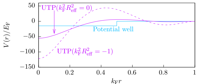
FIG. 2. (Color online) Plot of the potential well (blue), the UTP for the contact interaction (k_F R_{\text{eff}})^2 = 0 (solid purple), and the UTP for finite effective range (k_F R_{\text{eff}})^2 = -1 (dashed purple), normalized by the reciprocal Fermi energy E_F as a function of the dimensionless radius. All potentials are calibrated for interaction strength \ln(k_F a) = 0 .
