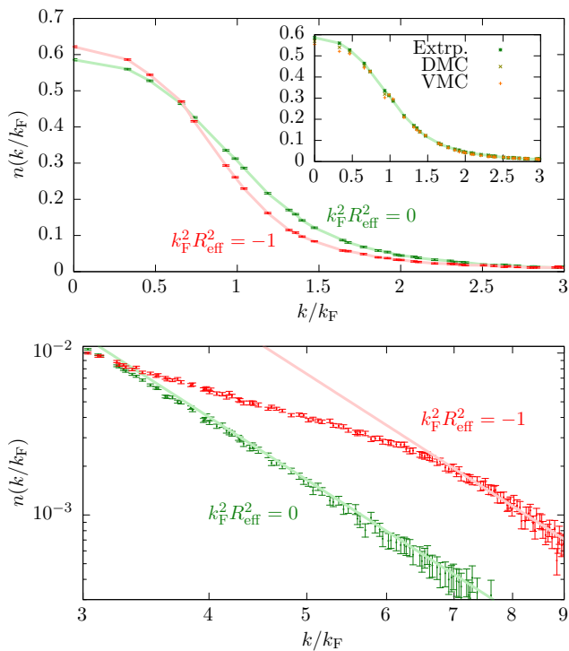
FIG. 9. (Color online) (Top) Extrapolated data for the momentum distribution n(k) for k_F^2 R_{\text{eff}}^2 \in \{0, -1\} . The inset additionally shows DMC, VMC, and extrapolated results separately for k_F^2 R_{\text{eff}}^2 = 0 . (Bottom) Tail of the momentum distribution on logarithmic axes, with the lines indicating n(k) \sim 1/k^4 .
