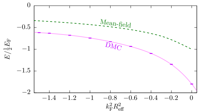
FIG. 7. (Color online) DMC ground-state energy per particle in units of that of a noninteracting gas as a function of the dimensionless effective range squared k_F^2 R_{\text{eff}}^2 shown by the solid purple line. The mean-field result is shown by the dashed green line.
