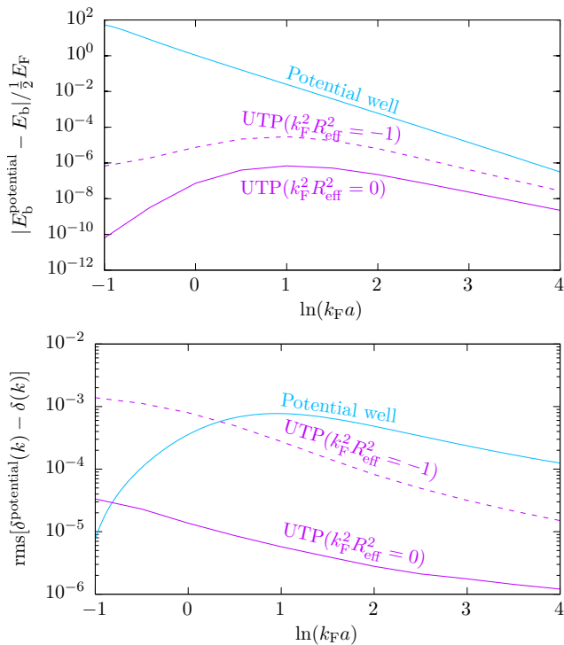
FIG. 3. (Color online) (Top) Difference in absolute value of the bound-state energy of the potential and the exact bound-state energy of the potential well (blue), the UTP for the contact interaction (k_F R_{\text{eff}})^2 = 0 (solid purple), and the UTP for finite effective range (k_F R_{\text{eff}})^2 = -1 (dashed purple). (Bottom) Root mean square (rms) scattering phase-shift error of the same potentials, with k averaged over the interval from 0 to the Fermi momentum k_F .
