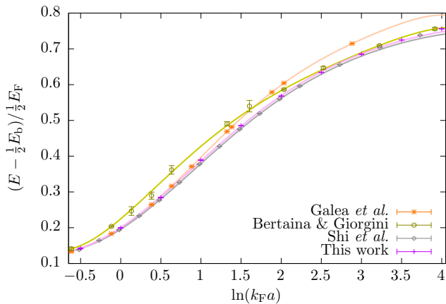
FIG. 4. (Color online) Ground-state energy per particle minus half the two-body binding energy, divided by the energy per particle in a noninteracting gas, as a function of the interaction parameter \ln(k_F a) across the BEC-BCS crossover. Next to our result we show the results from Refs. [21–23].
