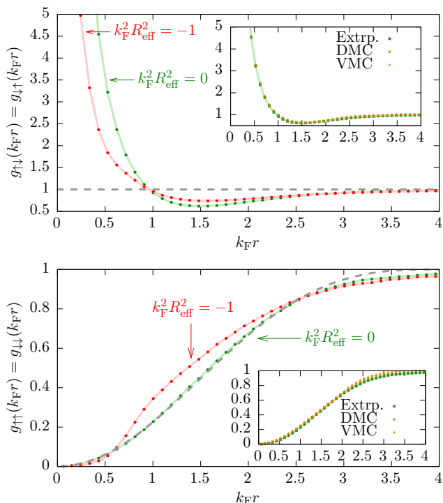
FIG. 10. (Color online) Pair-correlation function for opposite (top) and equal (bottom) spins for k_{\text{F}}^2 R_{\text{eff}}^2 \in \{-1, 0\} . The noninteracting correlation function for fermions is indicated by the gray dashed line. The insets show DMC, VMC, and extrapolated data separately.
