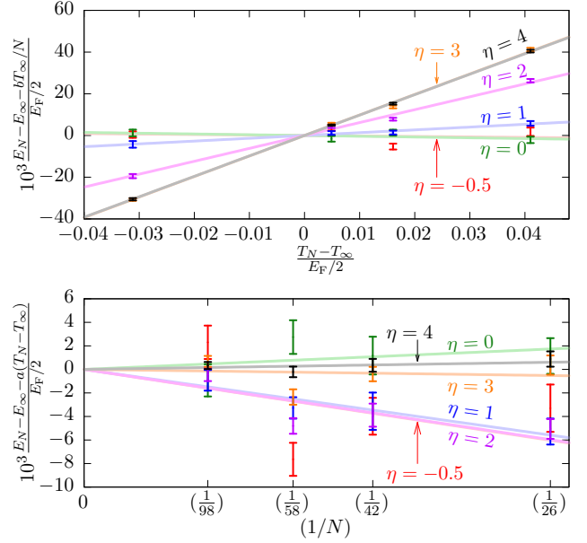
FIG. 12. (Color online) Variation of the dimensionless ground-state energy per particle with the difference in the noninteracting kinetic energy for a finite and infinite system (top) and the number of particles (bottom) for various interaction parameters \eta = \ln(k_F a) in the zero effective-range limit k_F^2 R_{\text{eff}}^2 = 0 . The straight lines show a weighted least squares fit to the data points.
