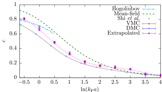
FIG. 6. (Color online) Condensate fraction as a function of the interaction parameter \ln(k_F a) . We show the VMC, DMC and extrapolated estimates, along with the auxiliary-field quantum Monte Carlo result from Shi et al. [22]. Also shown are the perturbative Bogoliubov theory for the BEC limit [56] and the mean-field prediction [57].
