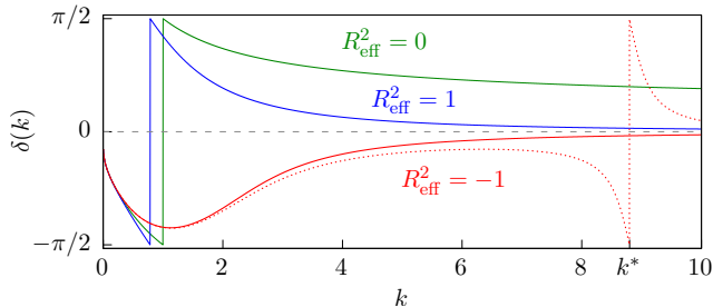
FIG. 1. (Color online) Scattering phase shift \delta(k) for a = 1 and R_{\text{eff}}^2 = \{-1, 0, 1\} (all lengths are in units of inverse momentum). For R_{\text{eff}}^2 = -1 the phase shift of a realistic potential with the same low-energy scattering properties is indicated by the red dotted line. The noninteracting phase shift is shown by the grey dashed line.
