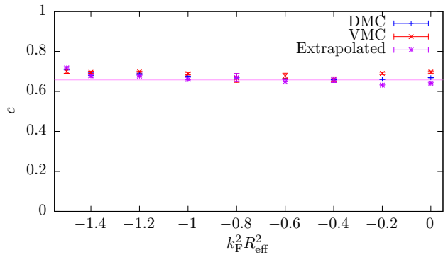
FIG. 8. (Color online) Condensate fraction as a function of the dimensionless effective range squared. We show the extrapolated result, as well as the bare VMC and DMC estimates.
