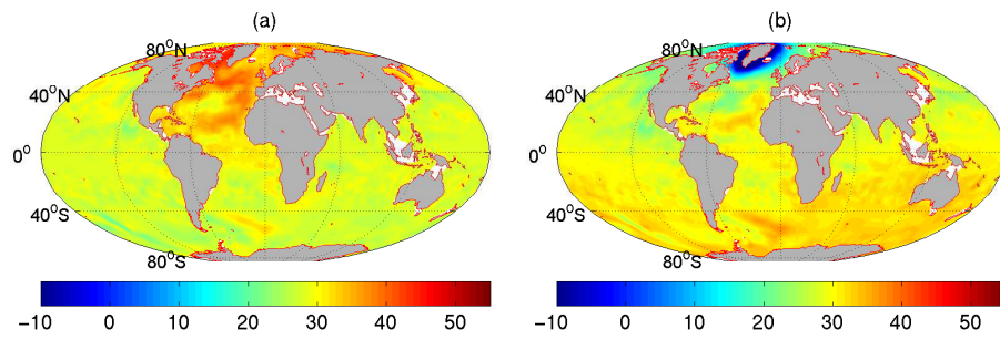
Figure 5: Sea level change (mm) with respect to the reference model simulation resulting from the Greenland Ice Sheet melting at a rate of 200 Gt/yr after 48 years; (a) sea level change with respect to an undisturbed geoid including regional and global mean sea level change and (b) sea level change with respect to the adjusted geoid as seen from altimetry after adding the gravitational effect due to Greenland ice mass loss
