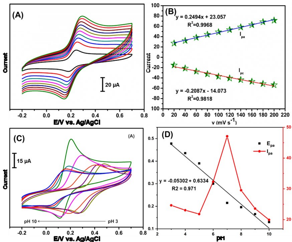
Figure 5 A) The effect of scan rate on the cyclic voltammetric response of GO-CMF/PdSPs composite modified GCE at 10 \mu\text{M} DA containing pH 7.0; the scan rate tested from 20 to 200 mV/s (inner to outer). B) The linear plot for the scan rate vs. anodic ( I_{pa} ) and cathodic ( I_{pc} ) current response. C) The voltammetric response of GO-CMF/PdSPs composite modified GCE at 10 \mu\text{M} DA containing different pH (pH 3 to 11) at a scan rate of 50 mV/s. D) Corresponding plot for pH vs. anodic peak potential ( E_{pa} ) and peak current ( I_{pa} ) of DA.
