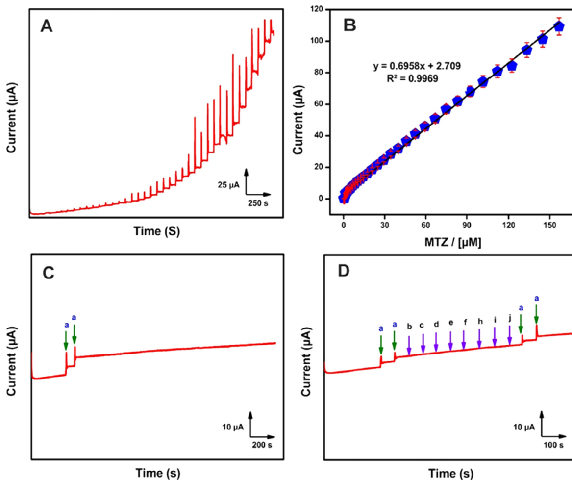
Fig. 7. (A) Amperometric response of GR- \beta -CD/CuO NPs composite modified RDE upon successive addition of various concentration of MTZ (0.002–210.0 \mu\text{M} ) into \text{N}_2 saturated pH 7.0. Working potential = -0.6 V. (B) The calibration curve for [MTZ] vs. amperometric current. (C) Amperometric response of GR- \beta -CD/CuO NPs composite modified RDE for the addition of 500 nM MTZ (a) and the current background response up to 2000 s. (D) Amperometric response of GR- \beta -CD/CuO NPs composite modified RDE for addition of 50 nM MTZ (a) and 20-fold additions of (b) 4-nitrophenol, (c) nitrobenzene, (d) nilutamide, (e) glucose, (f) dopamine, (g) glutaric acid, (h) serotonin, (i) histidine and (j) flutamide.
