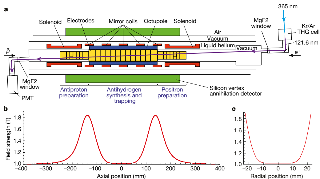
Fig. 1 | Experimental set-up. a , The three-layer silicon vertex annihilation detector is shown schematically in green; the external solenoid magnet for the Penning trap is not shown in this diagram. Laser light enters from the positron ( e^+ ) side (right) and is transmitted to the antiproton ( \bar{p} ) side (left) through vacuum-ultraviolet-grade MgF 2 ultrahigh-vacuum windows. The laser beam crosses the trap axis at an angle of 2.3°. The transmitted 121.6-nm pulses are detected by a photomultiplier at the antiproton side. b , Axial magnetic well formed by the five mirror coils and responsible for the axial confinement of cold (less than 0.5 K) anti-atoms. c , Radial magnetic octupole field profile. PMT, photomultiplier tube; THG, third-harmonic generation.
