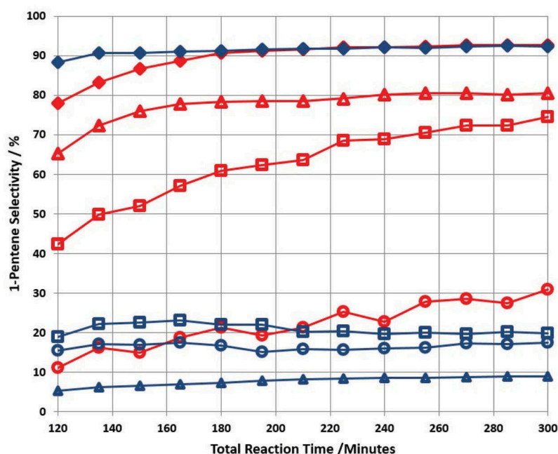
Figure 3. Comparison of catalytic performance in the selective hydrogenation of 1-pentyne to 1-pentene during extended operation at a fixed temperature, 240^\circ\text{C} . The chart shows \text{Pd}/\alpha\text{-Al}_2\text{O}_3 (blue) and \text{Pd}/\text{TiO}_2 (red) catalysts prepared by gas-phase cluster deposition (diamonds), deposition precipitation (squares), impregnation (circles), or ion exchange (triangles). The table summarizes the 1-pentyne conversion and 1-pentene selectivity after a dwell time of 180 min.
