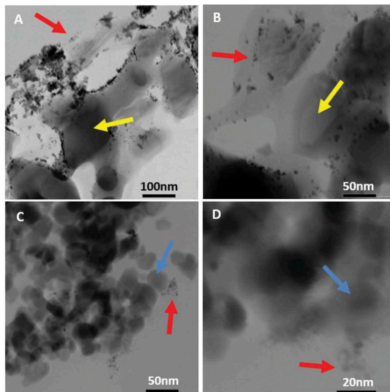
Figure 1. Representative bright-field aberration-corrected STEM images of the catalysts prepared by gas-phase cluster deposition: (A)–(B) Pd/ \alpha -Al 2 O 3 ; (C)–(D) Pd/TiO 2 . Examples of palladium particles are indicated by red arrows, alpha alumina particles with yellow arrows, and titania particles with blue arrows.
