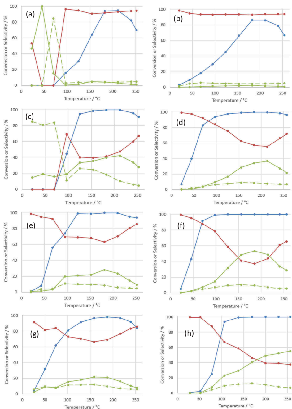
Figure 2. Catalyst testing in 1-pentyne hydrogenation. The 1-pentyne conversion is shown in blue, with selectivity to 1-pentene (red), 2-pentenes (green, solid line), and pentane (green, dashed line) also shown. The catalysts are (a) Pd/TiO 2 GCD; (b) Pd/ \alpha -Al 2 O 3 GCD; (c) Pd/TiO 2 impregnation; (d) Pd/ \alpha -Al 2 O 3 impregnation; (e) Pd/TiO 2 deposition-precipitation; (f) Pd/ \alpha -Al 2 O 3 deposition-precipitation; (g) Pd/TiO 2 ion exchange; and (h) Pd/ \alpha -Al 2 O 3 ion exchange.
