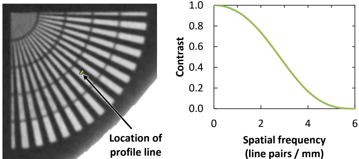
Figure 17. (a) Neutron radiograph of 'Siemens star' and location of profile line (green) used to calculate modulation transfer function. (b) Plot showing contrast with respect to spatial frequency. This curve is used to calculate the modulation transfer function and thus infer the theoretical minimum resolvable feature.
