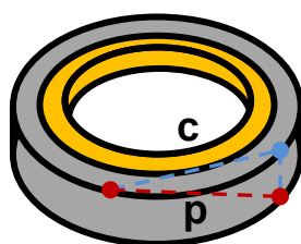
Figure 9. Schematic showing maximum chord length, c , through tungsten section of ROI samples and maximum attenuation path, p .
