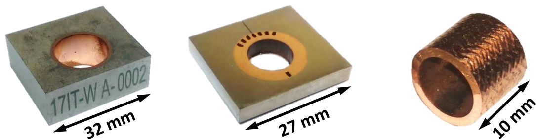
Figure 1. Three sample types used for this work: (left) ITER reference monoblock (ITER_MB), (centre) Culham Centre for Fusion Energy thermal break concept monoblock (CCFE_MB) and (right) Max-Planck-Institut für Plasmaphysik tungsten fibre / copper matrix coolant pipe (IPP_Wf-Cu)
