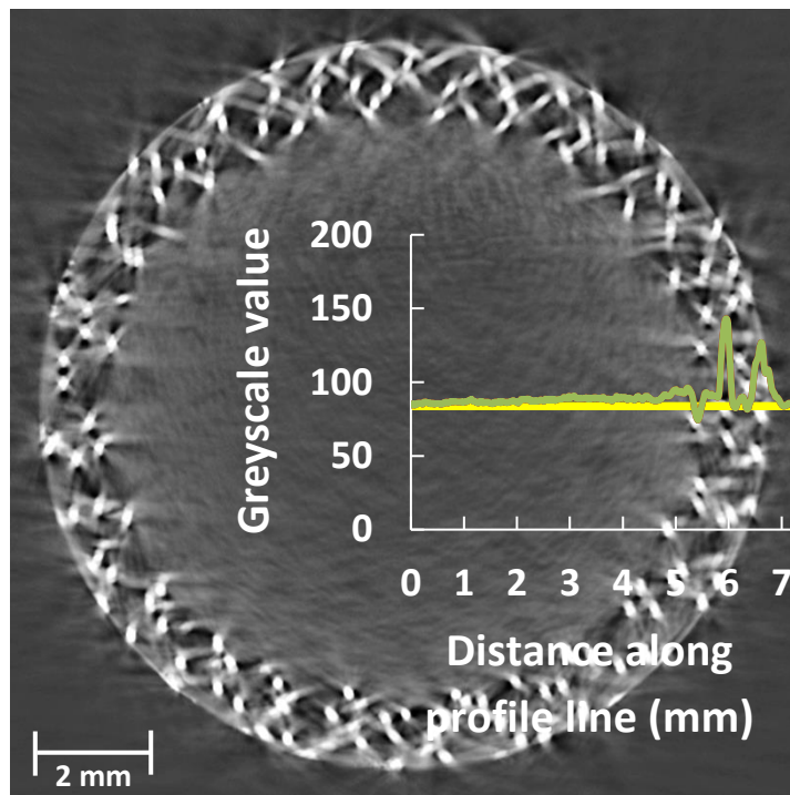
Figure 14. Plot of greyscale values (green) with respect to distance along profile line (yellow). Plot is overlaid on X-ray tomographic slice where profile was taken to show direct relation between changes in greyscale and image features.
