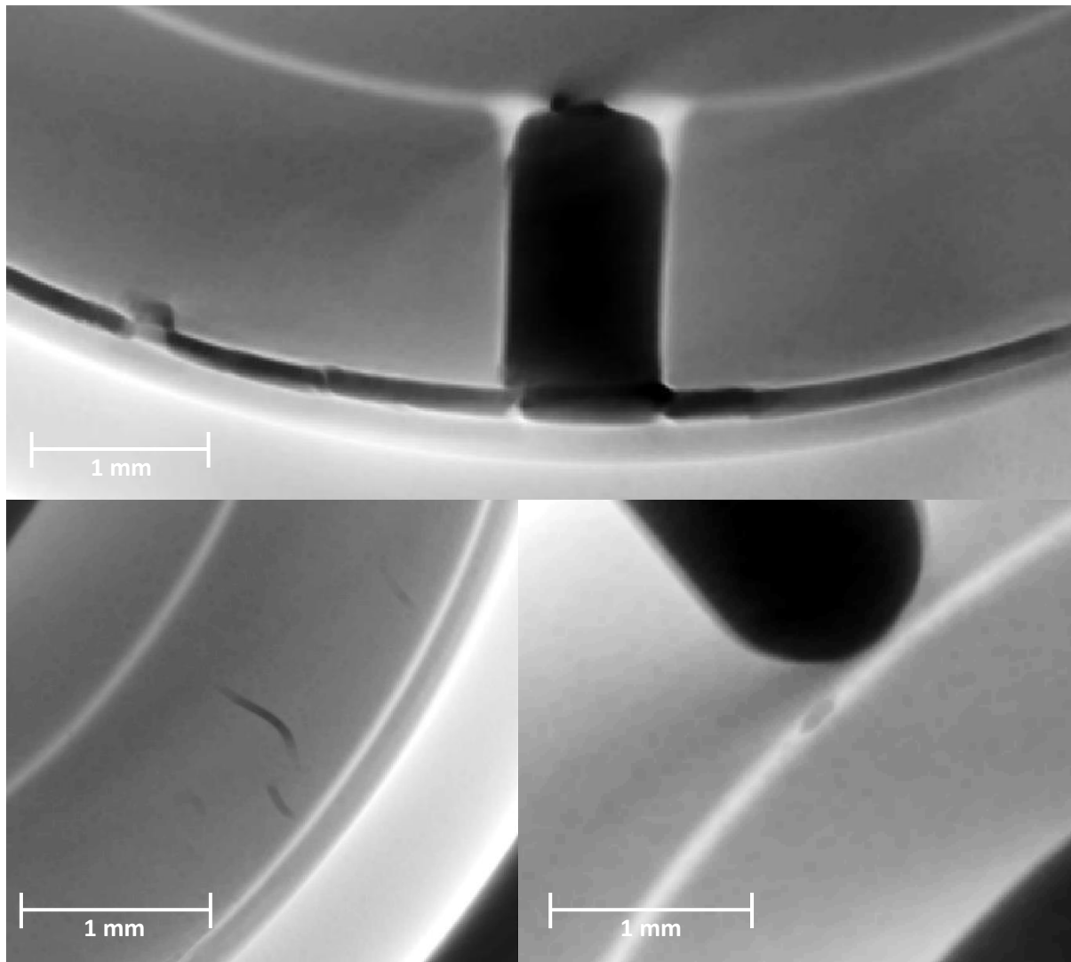
Figure 10. Zoomed in xy plane images from a X-ray tomography image of the CCFE_MB_ROI sample showing (top) debonding and variation in braze layer thickness, (bottom left) radial micro-cracking in Cu interlayer and (bottom right) pore within braze layer.
