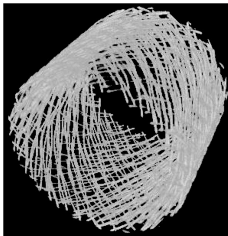
Figure 15. 3D visualisation from X-ray tomography data of W fibre placement within IPP_Wf-Cu sample, Cu matrix has been made transparent to assist viewing.
