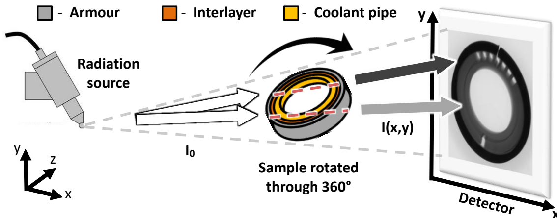
Figure 2. Schematic of X-ray tomography setup. Each detector pixel detector sums the signal attenuation along a particular path. Back projection algorithms use 2D radiographs taken through 360° to resolve the attenuation in 3D space. The main difference with neutron scanning is that the beam is quasi-parallel rather than having a cone angle.
