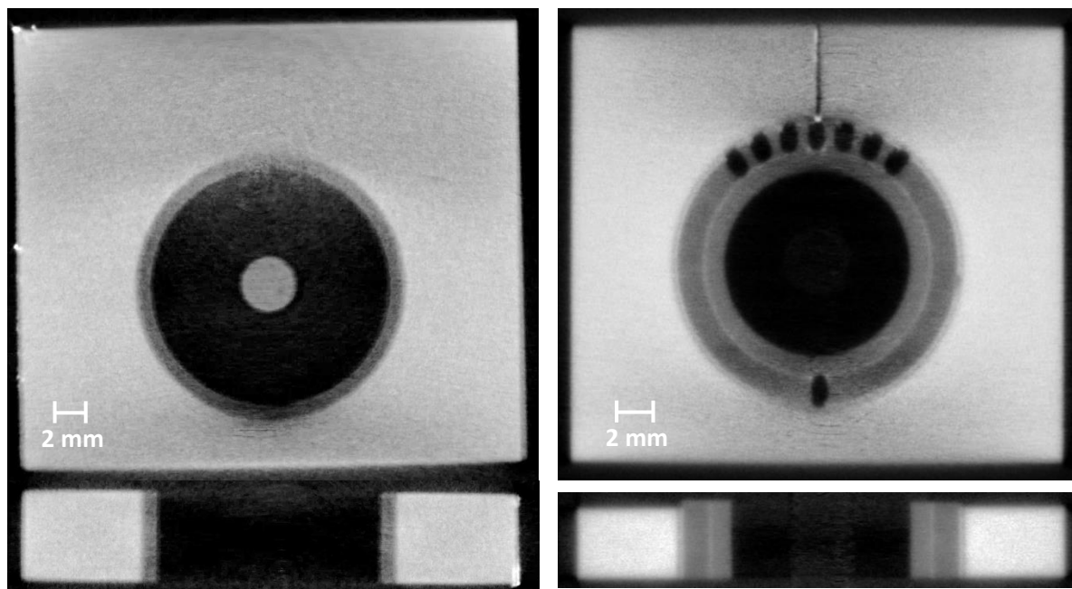
Figure 8. Example cross sectional neutron tomography data slices from the xy (top) and xz (bottom) planes for the ITER_MB (left) and CCFE_MB (right) samples.
