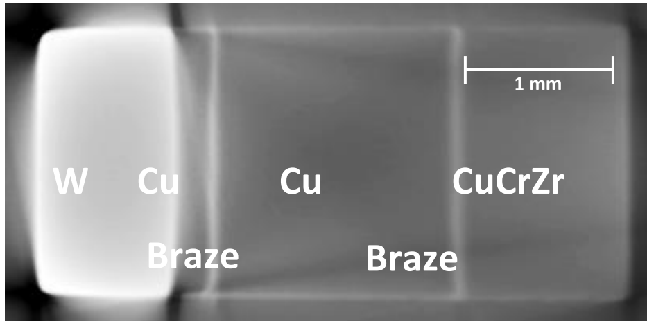
Figure 12. Zoomed in xz plane image from a X-ray tomography image of the CCFE_MB_ROI sample.
