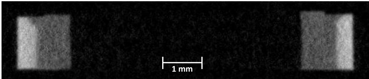
Figure 22. Cross sectional neutron tomography slices from the xz plane for the ITER_HHFT_ROI sample.
