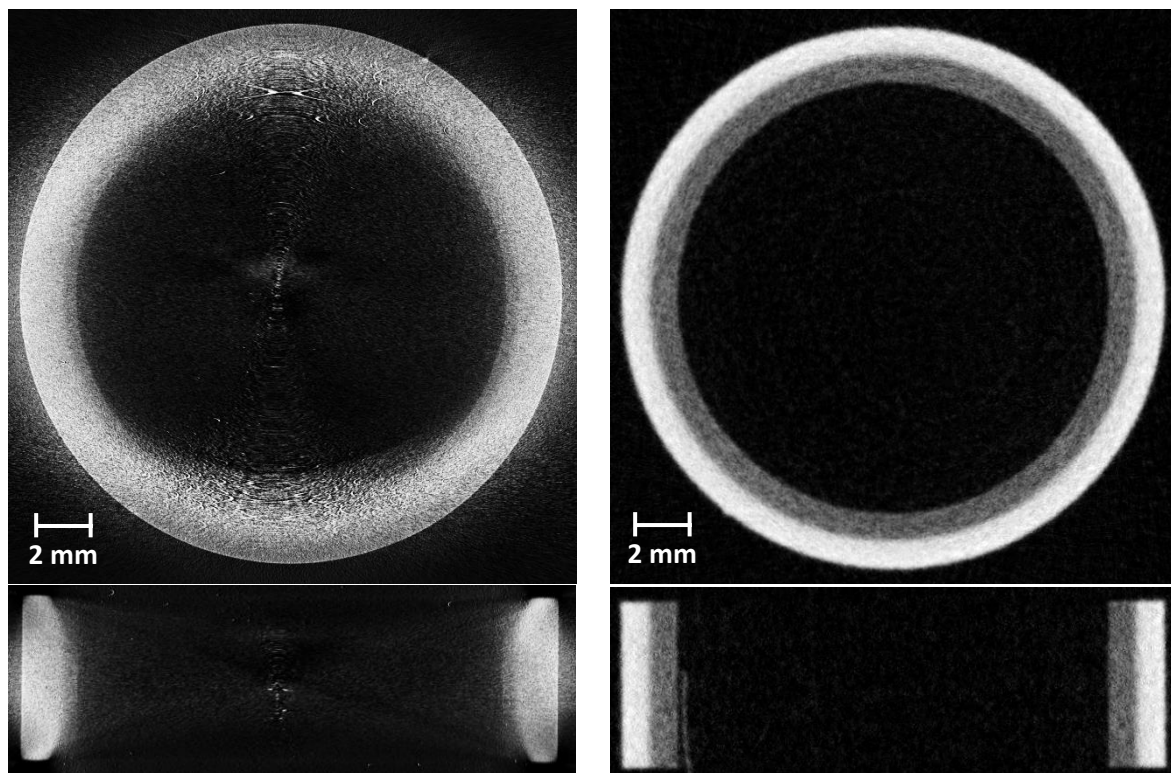
Figure 4. Example cross sectional tomography data slices from the xy (top) and xz (bottom) planes for the ITER_MB_ROI sample with a comparison of X-ray (left) vs. neutron (right) tomography imaging results.
