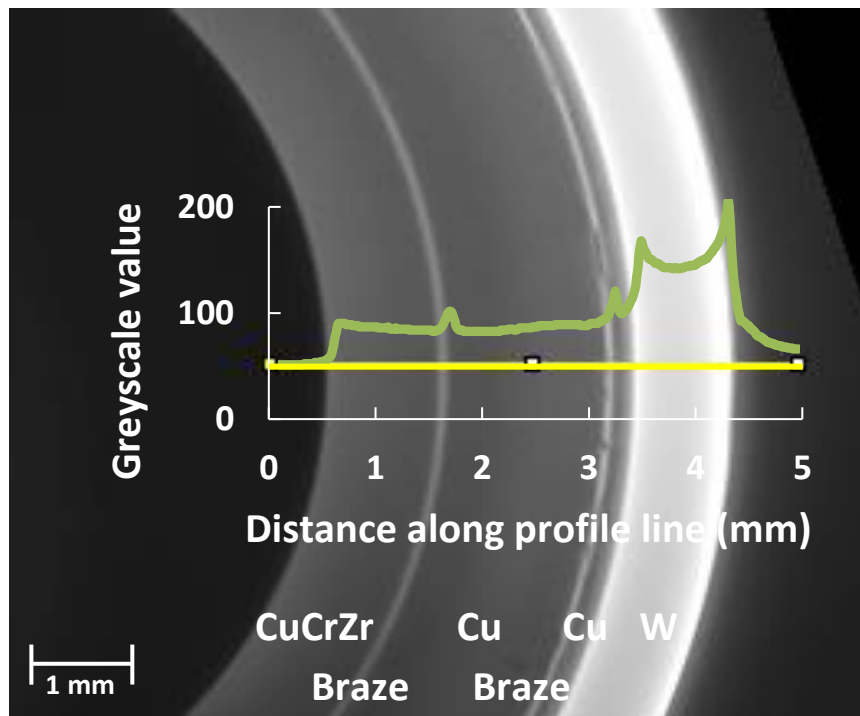
Figure 11. Plot of greyscale values (green) with respect to distance along profile line (yellow). Plot is overlaid on tomographic slice where profile was taken to show direct relation between changes in greyscale and image features.
