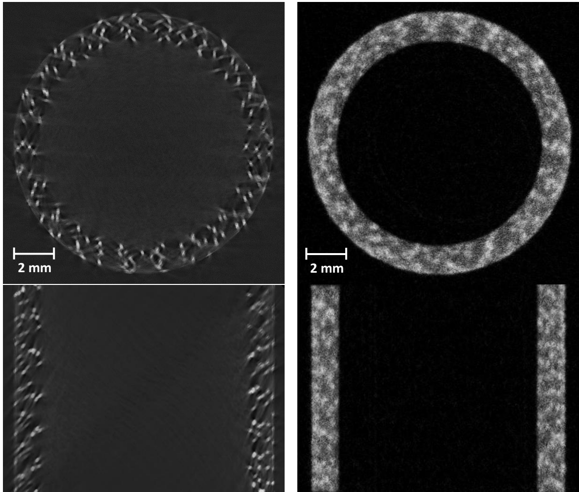
Figure 7. Example cross sectional tomography data slices from the xy (top) and xz (bottom) planes for the IPP_Wf-Cu sample with a comparison of X-ray (left) vs. neutron (right) tomography imaging results.
