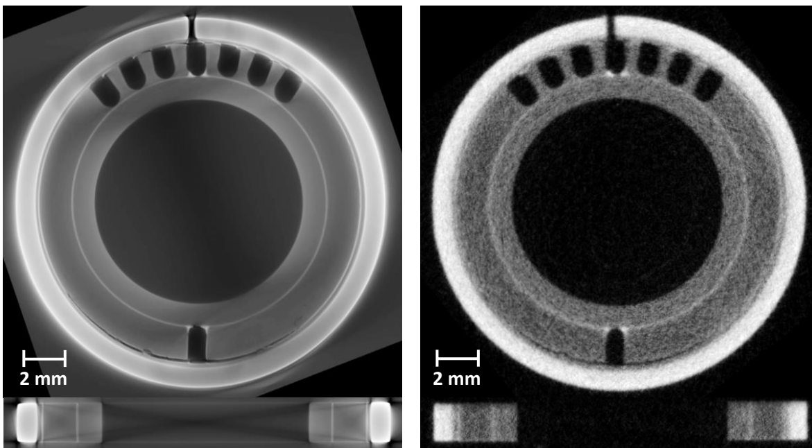
Figure 6. Example cross sectional tomography data slices from the xy (top) and xz (bottom) planes for the CCFE_MB_ROI sample with a comparison of X-ray (left) vs. neutron (right) tomography imaging results.
