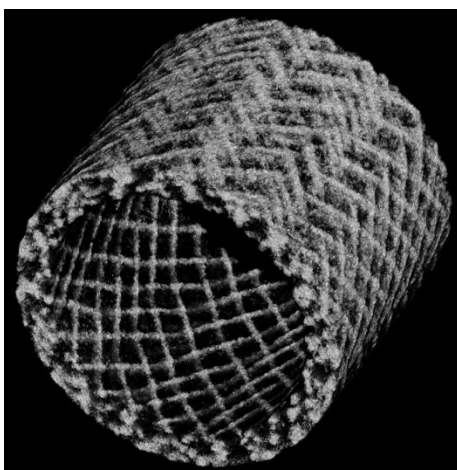
Figure 25. 3D visualisation from neutron tomography data of W fibre placement within IPP_Wf-Cu sample, Cu matrix has been made transparent to assist viewing.
