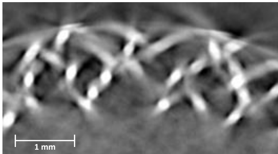
Figure 13. Zoomed in xy plane image from X-ray tomography image of IPP_Wf-Cu sample demonstrating that individual fibres are resolvable to locate positioning. Also shown is a lack of contrast between Cu matrix and background air; also streaking artefacts from W fibres are visible.
