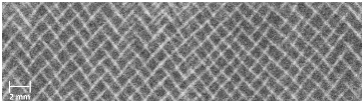
Figure 24. 'Unrolled' section from neutron tomography image of IPP_Wf-Cu sample at radius = 5.75 mm (i.e. x-axis is along \theta and y-axis is along length of pipe).
