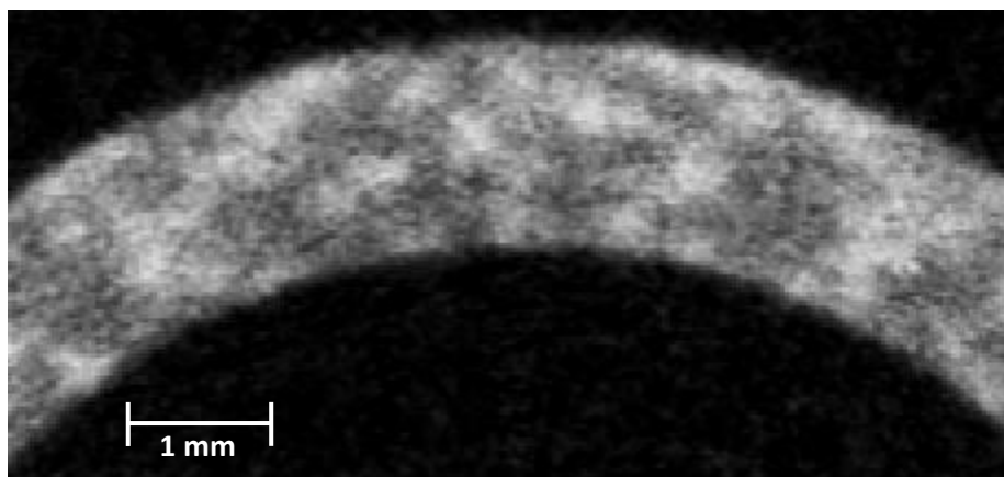
Figure 23. Zoomed in xy plane image from neutron tomography image of IPP_Wf-Cu sample.
