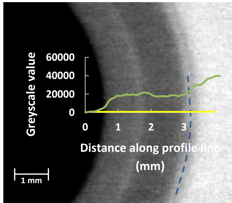
Figure 18. Plot of greyscale values (green) with respect to distance along profile line (yellow). Plot is overlaid on neutron tomographic slice where profile was taken to show direct relation between changes in greyscale and image features. Also shown is (dashed blue) profile line used for Figure 19 to highlight void observed in braze layer.
