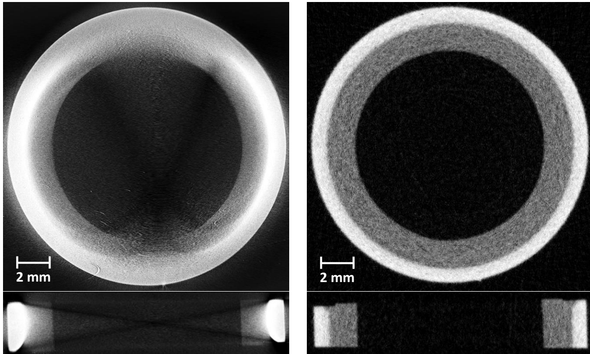
Figure 5. Example cross sectional tomography data slices from the xy (top) and xz (bottom) planes for the ITER_HHFT_ROI sample with a comparison of X-ray (left) vs. neutron (right) tomography imaging results.
