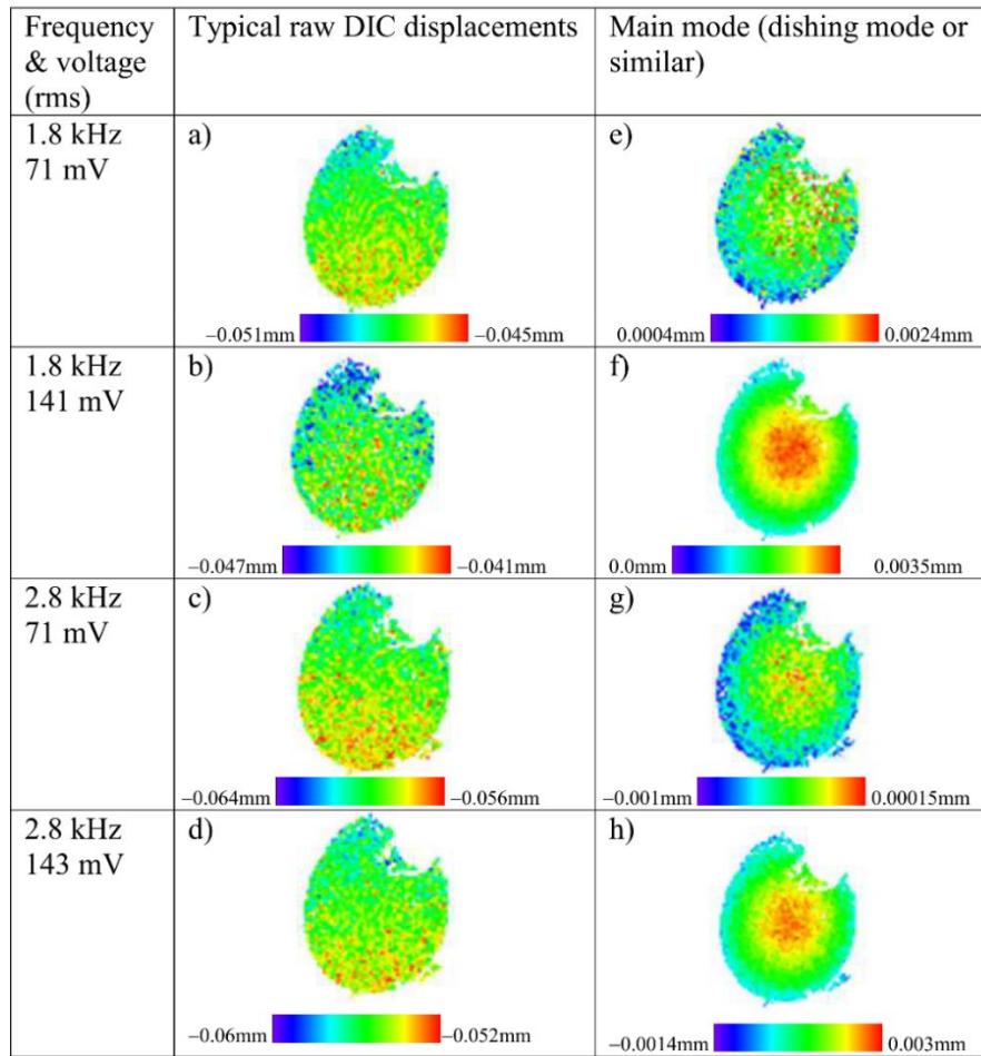
Figure 4: Results for polycrystalline (PZT) actuator: (a-d) typical raw deflected shapes from DIC system; (e-h) deflected shapes from DIC vibrometry using external reference signal. Note that no higher-order shapes were detected in quadrature with these deflections.
