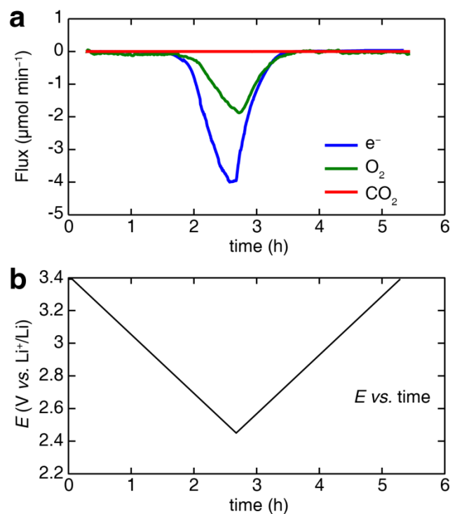
Figure 5 | In-situ DEMS in DBBQ-TEGDME showing 2.03 e^- per \text{O}_2 consumption, consistent with formation of \text{Li}_2\text{O}_2 . (a) discharge current (blue), \text{O}_2 consumption (green) and \text{CO}_2 evolution (red) in 10 mM DBBQ - 1 M LiTFSI in TEGDME; (b) voltage profile of the DEMS cell. Cyclic voltammetry was applied. e^-/\text{O}_2 ratio was obtained from the integral of charge passed and total \text{O}_2 consumption.
