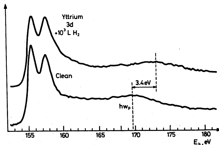
Fig. 3. 3d Core-level peaks of Y
