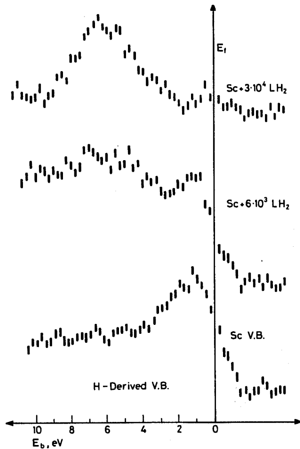
Fig. 2. The XPS valence band spectra of hydrogenated Sc
