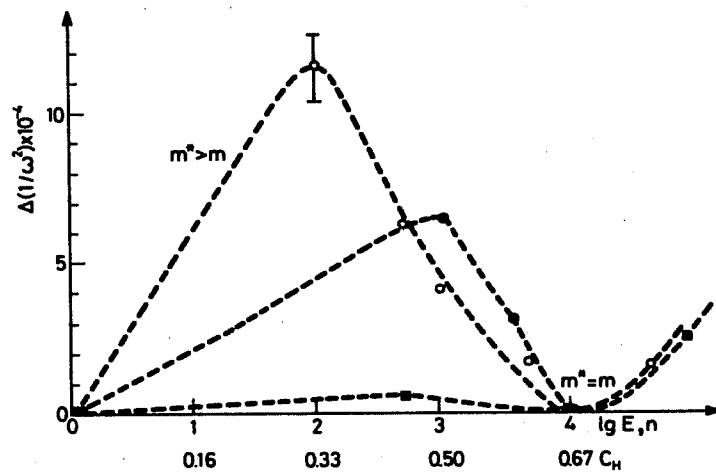
Fig. 5. The comorison of our result with data obtained for Ti (Lamartine et al. (1980)) ○ — Scandium, ■ — Yttrium, + — Titan For the magnification of the effect the shift in \omega^{-2} have been shown versus \lg E (or C_H )
