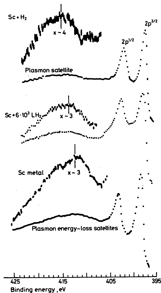
Fig. 1. The 2p XPS Core-level Spectra of Sc
