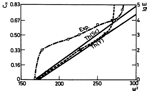
Fig. 4. The dependence of the plasmon energy by the hydrogen exposure ○ — Scandium, ■ — Yttrium, Th(Sc) and Th(Y) are the theoretically expected curves
