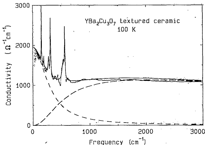
FIG. 1. The optical conductivity of the textured ceramic of \text{YBa}_2\text{Cu}_3\text{O}_{7-x} obtained by Kramers-Kronig transformation of the reflectance is shown as points. The smooth curve is a fit of the reflectance to a dielectric function that uses Lorentz oscillators to describe the phonons and a broad band for the midinfrared oscillator strength in addition to a Drude absorption centered on zero frequency. The dashed curves show individual contribution of the Drude and the midinfrared bands to the conductivity.
