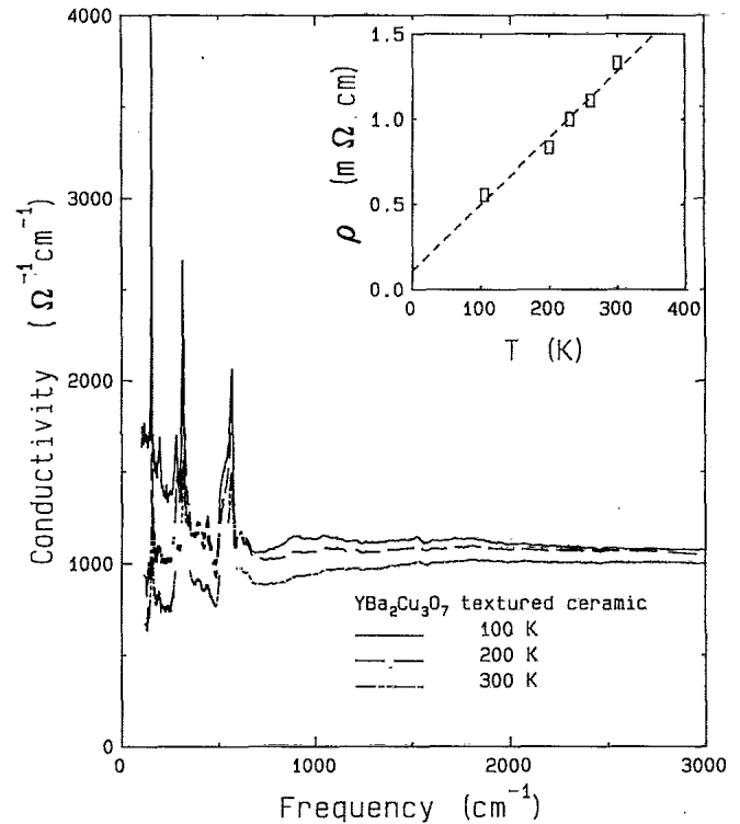
FIG. 2. Temperature dependence of the conductivity. Inset: the resistivity, measured by far-infrared means of 100 \text{ cm}^{-1} , as a function of temperature. It shows the characteristic linear resistivity of oxide superconductors. The amplitude of the broad midinfrared band at 2000 \text{ cm}^{-1} changes little with temperature.
