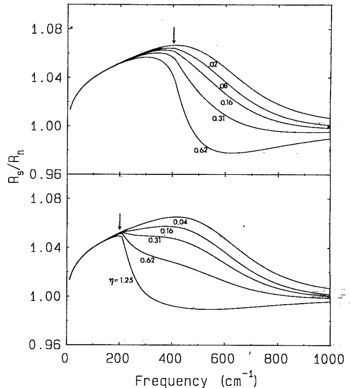
FIG. 5. Calculated reflectance ratio R_s/R_n for a BCS superconductor with 2\Delta/k_B T_c of 3.5 (bottom) and 7.0 (top) for various values of \eta = (2\tau\Delta)^{-1} . When this parameter is large the superconducting gap, shown as an arrow, can be seen in the reflectance ratio. For \eta \ll 1 the plasma maximum dominates the reflectance and the gap cannot be seen. The calculation uses the parameters from the normal-state fit to \text{YBa}_2\text{Cu}_3\text{O}_{7-\delta} shown in Fig. 3.
