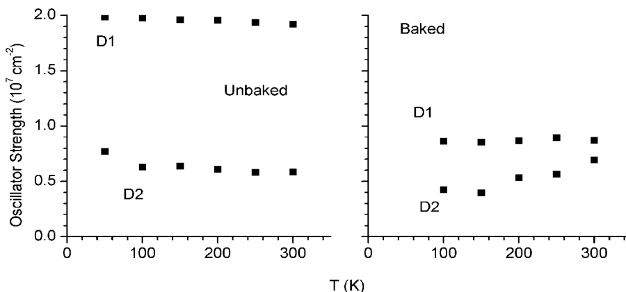
FIGURE 3. Temperature dependence of low-frequency oscillator strength in Sample 3 before and after baking.
