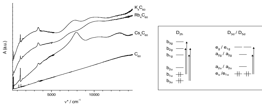
FIGURE 2. MIR and NIR spectrum of K_4C_{60} , Rb_4C_{60} and Cs_4C_{60} without background correction. Second panel shows the allowed transitions between the split molecular orbitals of the distorted fulleride ions leading to the observed peaks in the NIR. The ordering of the levels on this figure is arbitrary.
