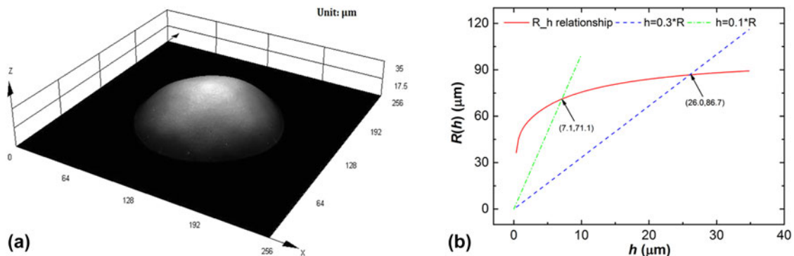
FIG. 6. (a) The geometrical surface of the spherical indenter tip measured by OLYMPUS OLS4000; (b) the equivalent radii of the spherical diamond indenter at various depths (solid line). The arrows mark the equivalent radii at h/R = 0.1 and h/R = 0.3 .
