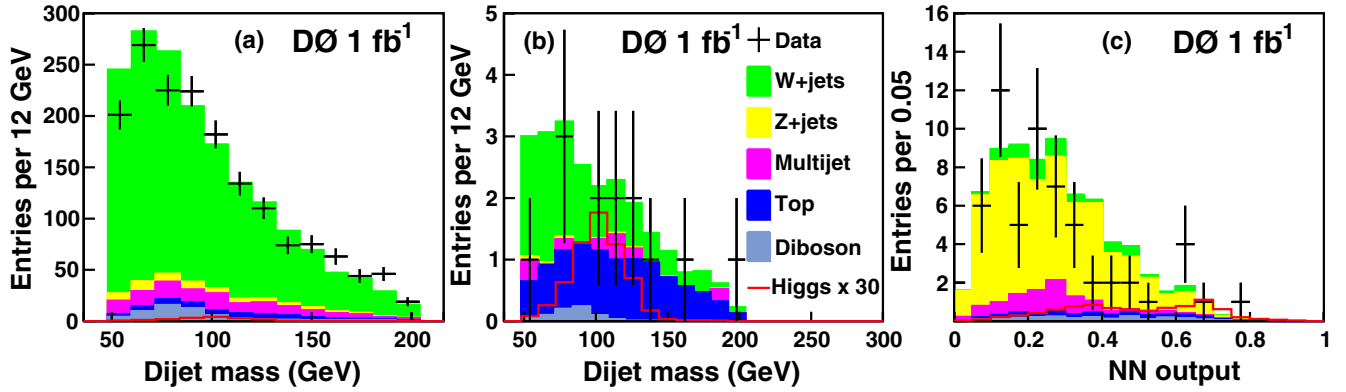
FIG. 1 (color online). The dijet mass distribution for all tau types for the \tau\nu analysis (a) before b tagging, and (b) after the final selection; (c) the combined NN_{Z\text{jets}} variable for the low Higgs boson mass \tau\tau analysis. The signal is shown (multiplied by 30) for M_H = 115 GeV.
