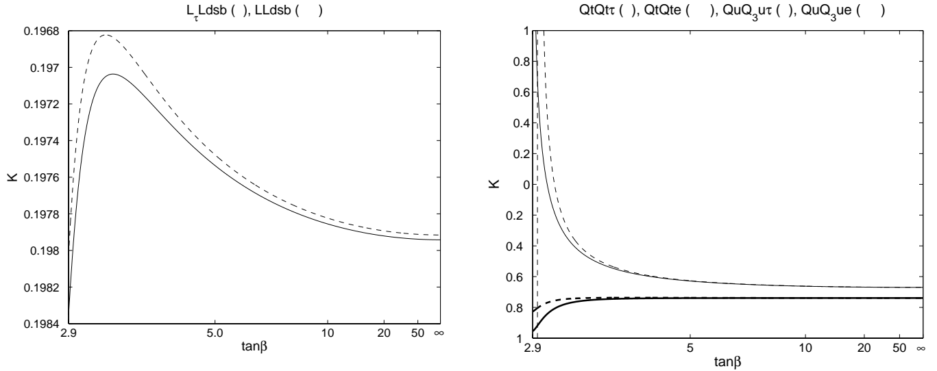
FIG. 2. K vs \tan\beta . On the left LLdsb flat direction with a choice of stau in the flat direction (solid line) and no stau in the flat direction (dashed line). On the right QuQue flat direction with u from 3rd generation (thick lines) and Q from 3rd generation (thin lines), e from 3rd generation (solid line) and e from 1st or 2nd generation (dashed line).
