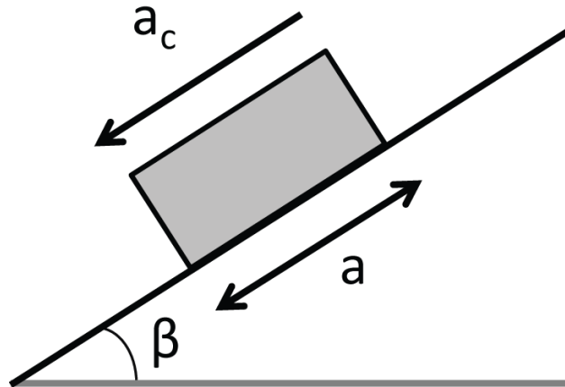
Figure 2-3 Illustration of the Newmark sliding block model, after (Jibson, 2011: 45), where a is the earthquake ground acceleration at the base of the block, a_c is the critical acceleration of the block, and \beta is the angle of inclination of the sliding surface.
