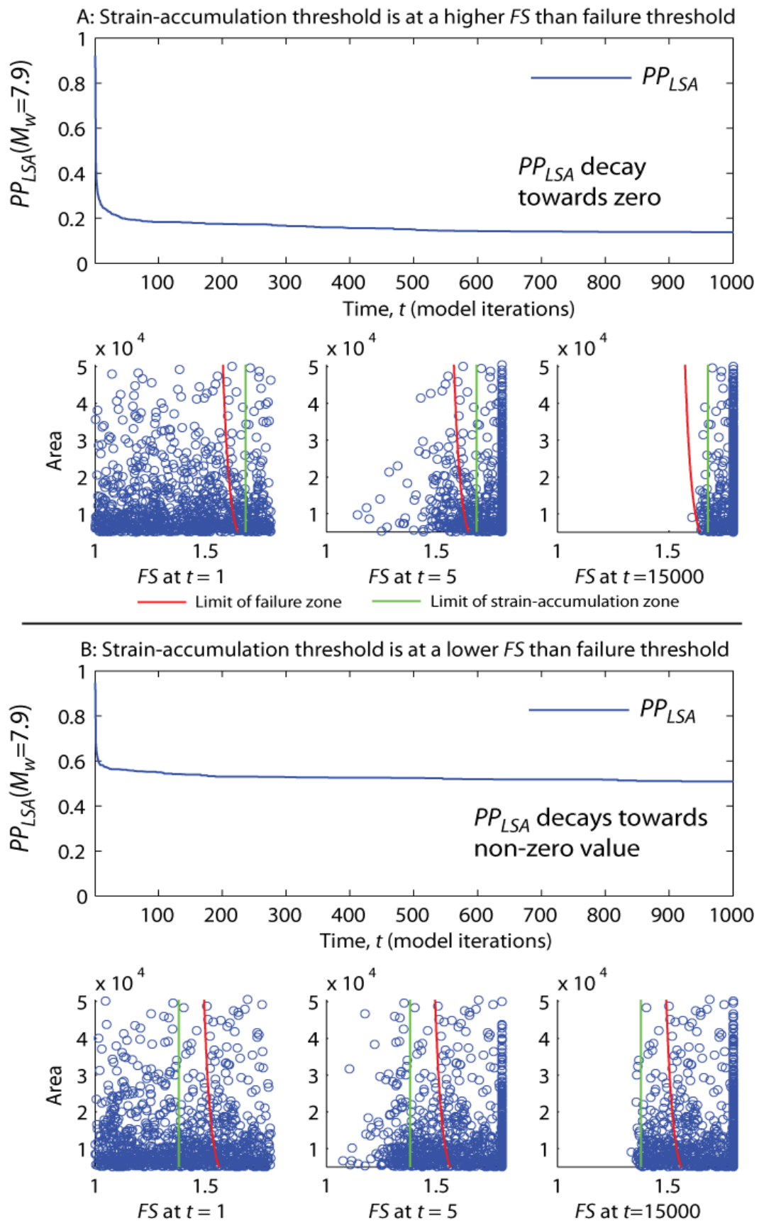
Figure 6-15 Model time series and FS-A plots, when subjected to a sequence of constant magnitude earthquakes, where PGA(Lm) < a_c(\tau_{fp}) . The FS-A space to the left of the green line is the strain-accumulation zone, while the space to the left of the red line is the failure zone. (A) where the strain-accumulation threshold is at a higher FS than the failure zone threshold, landslide propensity decays towards zero; (B) where the strain-accumulation threshold is at a lower FS than the failure zone threshold, landslide propensity decays towards a non-zero value
