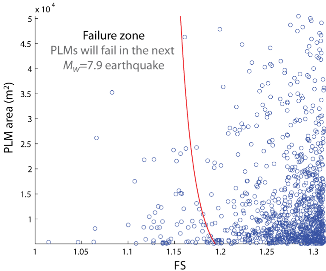
Figure 6-8 Model FS-Area space. Blue circles represent individual PLMs, which move from right to left on the plot as earthquakes exceed \alpha_c and PLMs progress through their failure cycle. The red line is the threshold of the failure zone (region to the left of the red line). When a M_w = 7.9 earthquake occurs, all PLMs within the failure zone undergo failure. PP_{LSA} is the total area of PLMs in the failure zone divided by the total area of PLMs. Note that the failure zone threshold is curved as smaller PLMs require less displacement to achieve the same strength decay as larger PLMs.
