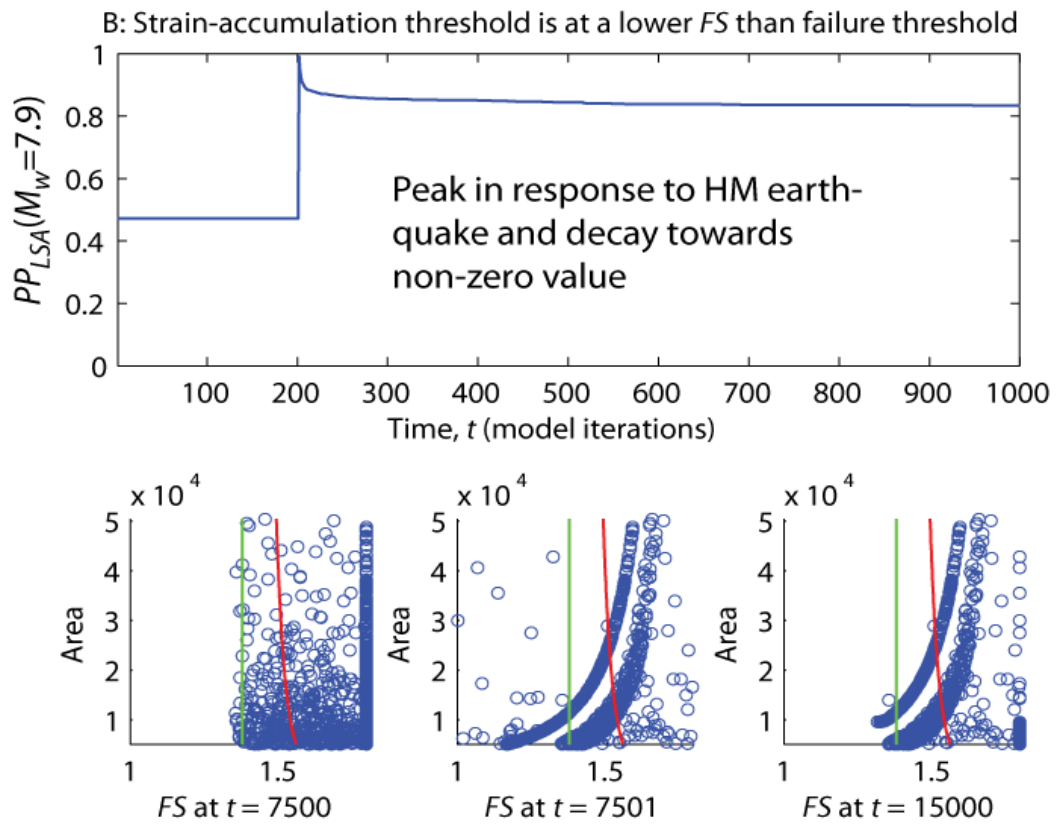
Figure 6-16 Model time series and FS-A plots, when subjected to a high magnitude earthquake, where PGA(L_m) < a_c(\tau_{fp}) . (A) where the strain-accumulation threshold is at a higher FS than the failure threshold; (B) where the strain-accumulation threshold is at a lower FS than the failure threshold
