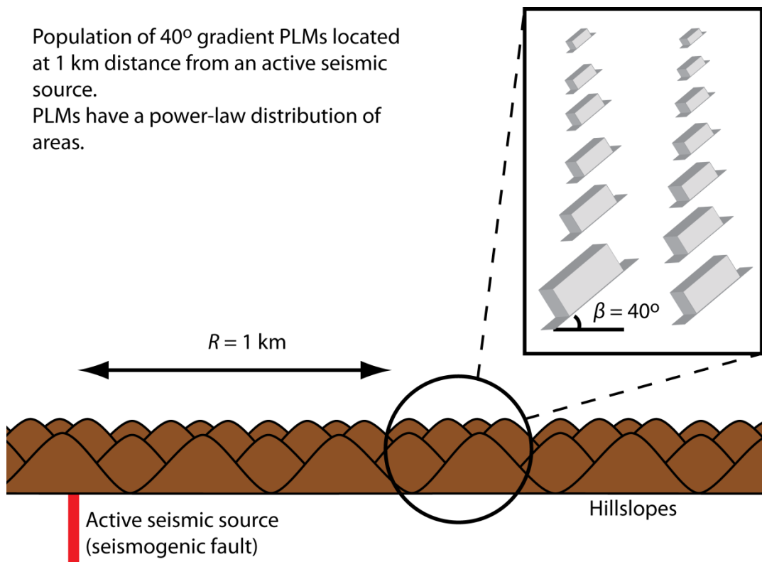
Figure 6-7 Schematic diagram of model experimental set-up. A population of Newmark sliding blocks represents the 40° hillslopes of a mountain range, located 1 km from an active seismic source.
