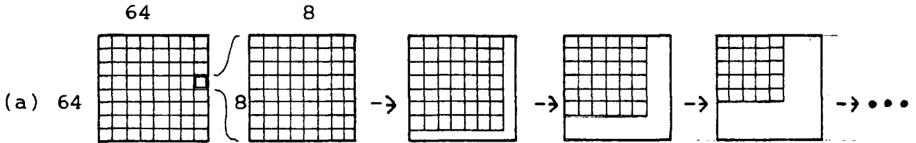
Figure 6.10: A parallel algorithm to compress a 64 x 64 image to an 8 x 8
