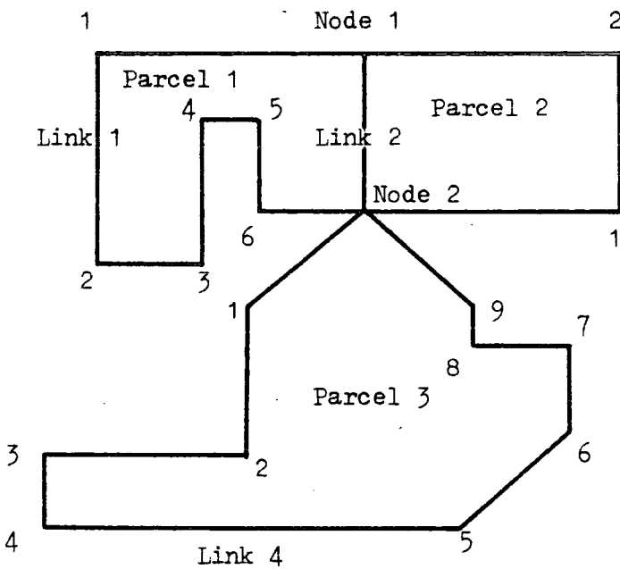
Figure 2·8: An example of the complex data base schema required to represent the simplest of vector link and node structures
