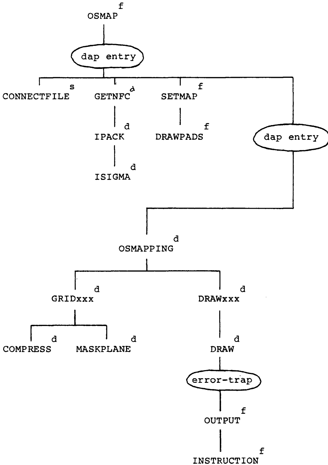
Figure 6.8: A block summary of the graphics routines developed for the DAP and listed in annex 6c
