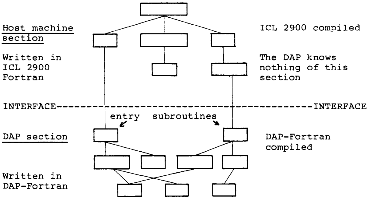
Figure 6.4 Block diagram showing the modular nature and the separation between host- and DAP-related sections of typical DAP software
