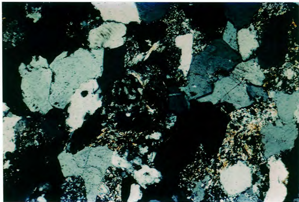
Plate 6.5 - Kaolinite/illite and opaque ?haematite cements in sandstone above Brockwell coal, Middridge Quarry. Length of photomicrograph 1.2mm. (Crossed polars).
