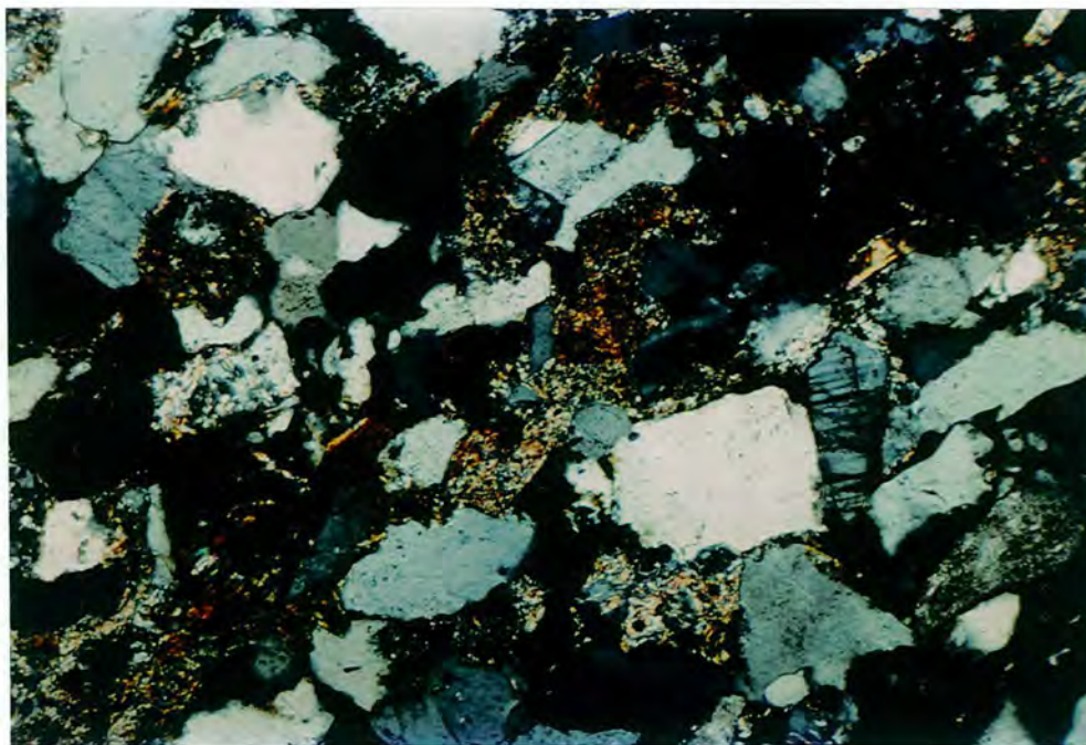
Plate 7.I4 - Photomicrograph of the "Low Main Post", showing abundance of kaolinite/illite cement. Length of photomicrograph 1.2mm. (Crossed polars).
