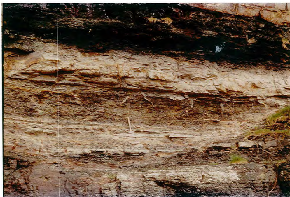
Plate II.8 - Palaeosol profile from the basal Westphalian A east of Amroth, Pembs. The profile contains abundant sphaerosiderite, and goethite- and sandstone-filled cracks (above hammer, 30cms long), and is overlain by a thin coal.
