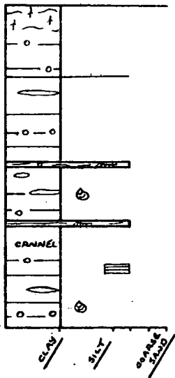
Quiet water claystones Sequences \leq 10m
