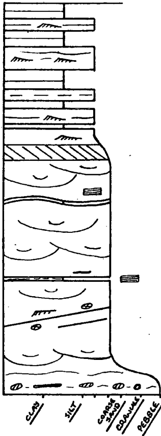
Major channel deposits. Sequences \leq 30m .
