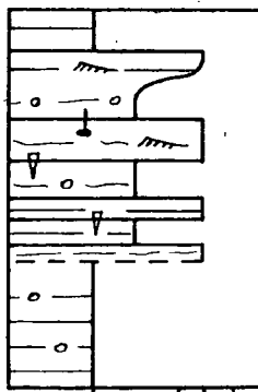
Distal feeder channel deposits. Sequences \leq 2m .
