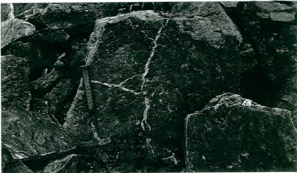
Plate 6.26 - Sandstone-filled desiccation cracks in root-penetrated sediment beneath the Bottom Tilley (PI02) coal, Buckhead O.C.C.S. Hammer is 30 cm long.
