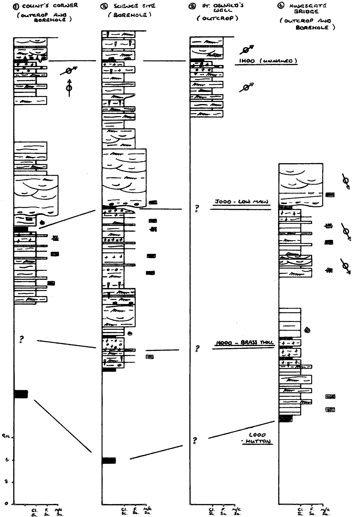
BASED ON SECTIONS 332, 325, 334 AND 335 RESPECTIVELY, AND I.C.S./UNIVERSITY BOREHOLE RECORDS. DETAILED PALAEOCURRENTS AND SECTION LOCATIONS ON FIG. 5.14.
