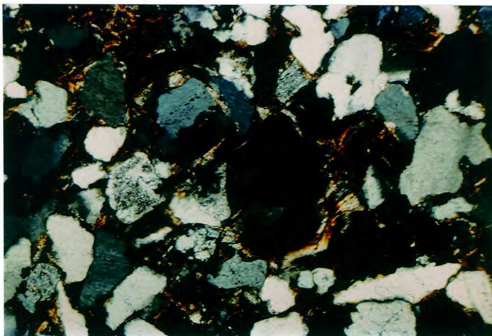
Plate 6.3 - Photomicrograph showing development of coarsely crystalline, authigenic kaolinite (centre of photo) in sandstone immediately underlying the Kays Lea Marine Band, West Butsfield Quarry. Length of photomicrograph 1.0mm. (Crossed polars).
