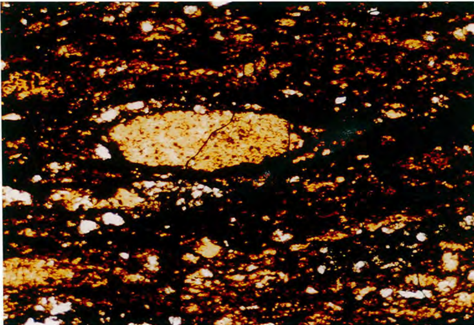
Plate 6.I6 - "Graupen" (granules) of microcrystalline kaolinite in kaolinitic claystone, Middle Tilley coal, Rowley O.C.C.S. Length of photomicrograph 1.2mm. (Plane polarized light).
