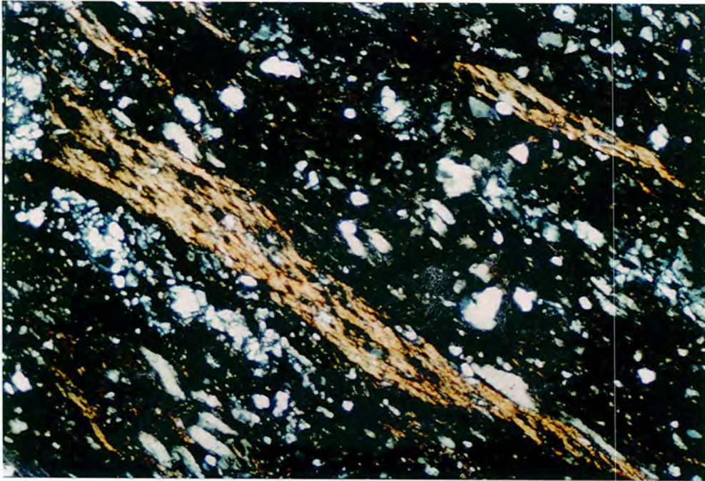
Plate 6.I7 - Kaolinite groundmass in kaolinitic claystone, showing preferred orientation (lamination), Middle Tilley coal, Rowley O.C.C.S. Length of photomicrograph 1.2mm. (Plane polarized light).
