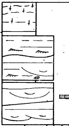
Minor crevasse channel deposits. Sequences \leq 2m . (COMMONLY VERTICALLY STACKED)
