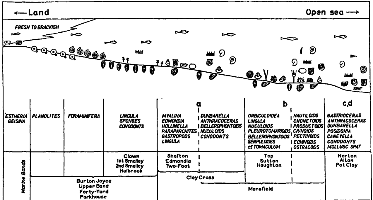
a) Idealized relationship of facies belts and their typical faunas ( Faunal phases ; a.- Myalina, b.- Productoid, c.- Pectinoid, d.- Goniatite ).
