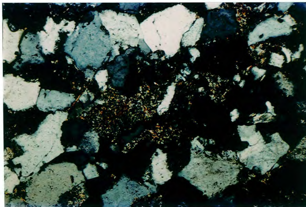
Plate 5.I - Photomicrograph of a typical Durham Coal Measure sandstone, showing the characteristic kaolinite/illitic mica cement association. Low Main Post, Croxdale Beck. Length of photomicrograph 1.2mm. (Crossed polars).
