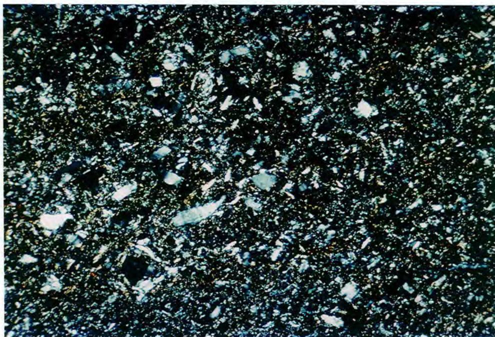
Plate 6.24 - Photomicrograph of Middle Tilley kaolinitic claystone from Mown Meadows O.C.C.S., showing common flecks of white mica. Length of photomicrograph 1.2mm. (Crossed polars)
