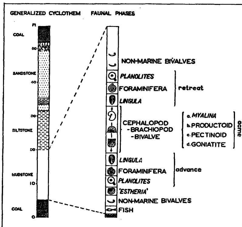
b) Vertical distribution of faunal phases associated with an idealized Westphalian marine incursion.
