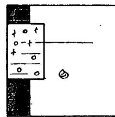
Passive lake margin deposits Sequences \leq 3m
