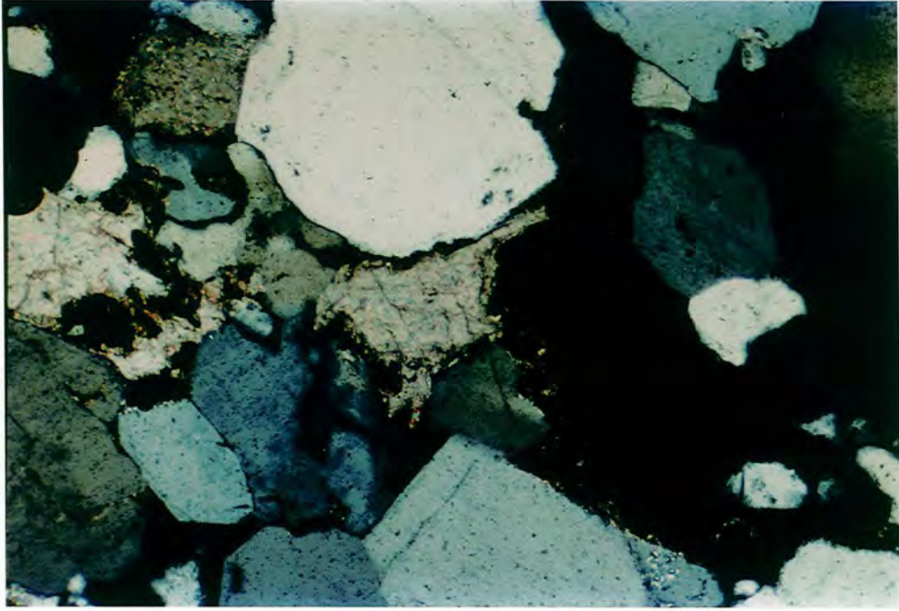
Plate 6.29 - Dolomite and pyrite/marcasite cements in sandstone from above the Bottom Tilley (PI02) coal at Buckhead O.C.C.S. Length of photomicrograph 1.2mm. (Crossed polars).
