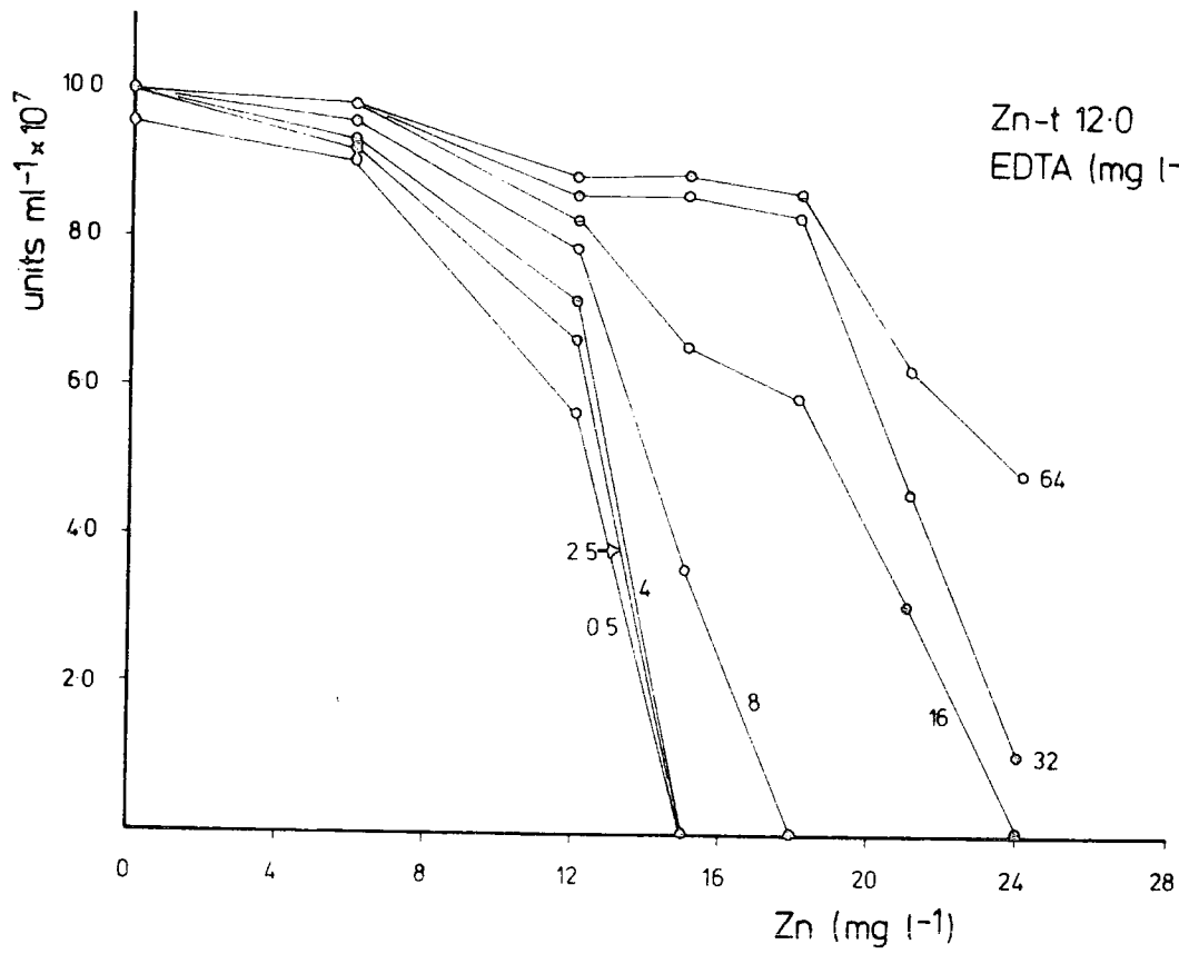
Fig. 5.13 Influence of EDTA on Zn toxicity to Zn-t12.0 Anacystis strain.
