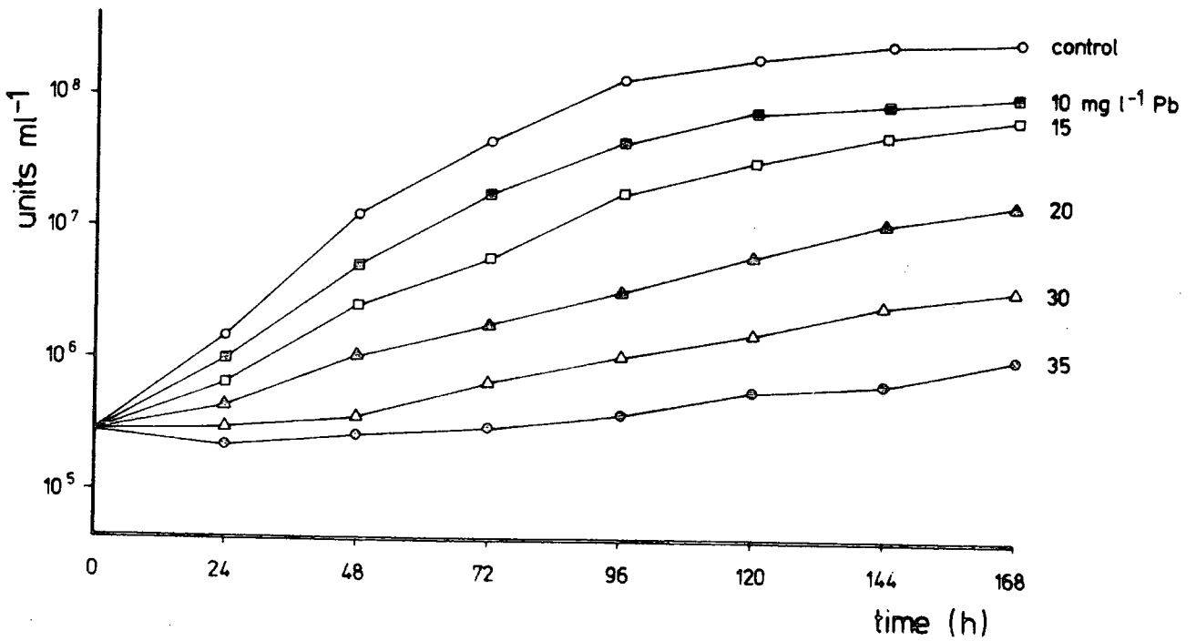
Fig. 4.31 Influence of Pb on growth of wild-type Anacystis .
