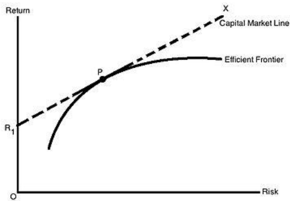
Figure 4.1: Efficient Frontier with Risk-Free Rate
