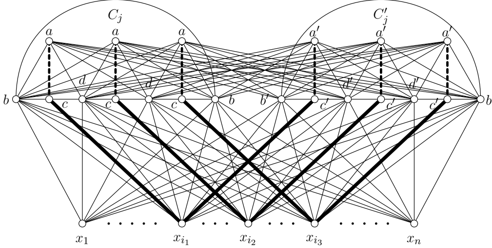
Figure 3.2: The graph G_I^* for the clause C_j = \{x_{i_1}, x_{i_2}, x_{i_3}\} .
