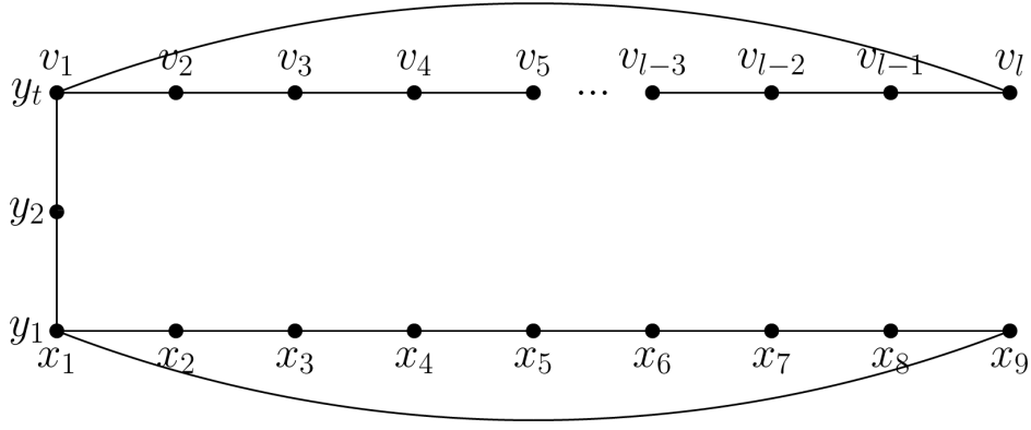
Figure 2.10: A subgraph of a P_{17} -free graph of girth 9.
