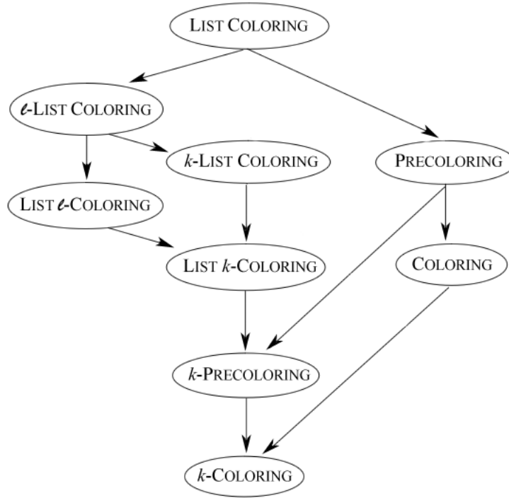
Figure 1.1: Relationships between COLOURING and its variants. An arrow from one problem to another problem indicates that the latter problem is a special case of the first one, whereas k and \ell are any two integers for which \ell \geq k .
