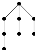
Figure 1.3: The graph S_{2,2,3}
