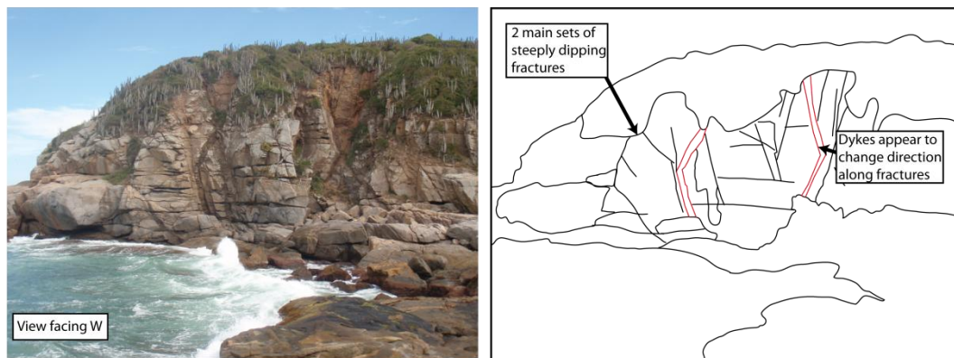
Figure 5.8A. Dykes seen in a cliff section at Praia das Conchas (locality Pc18). The dykes clearly follow the two main sets of fractures seen here (NW-dipping and SE-dipping), although they do not appear to be affected by shallowly dipping structures. These dykes are interpreted as having intruded along pre-existing fractures, as it is the simplest explanation for the close similarity in their geometries. Cliff is ~ 20m high
