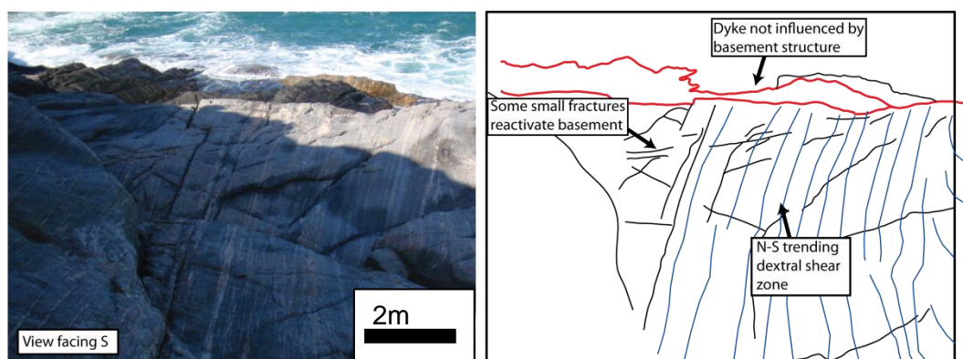
Figure 5.8C A N-S trending basement shear zone is seen at Praia das Conchas, cut by the large dyke. This relatively large basement structure has no control on the geometry of the dyke, although it does appear to have been reactivated by a small number of open fractures. Many other fractures simply cross-cut the shear zone. Most fractures do not cut the dyke, but a number of NNE-SSW trending fractures do (Fig. 5.8B).
