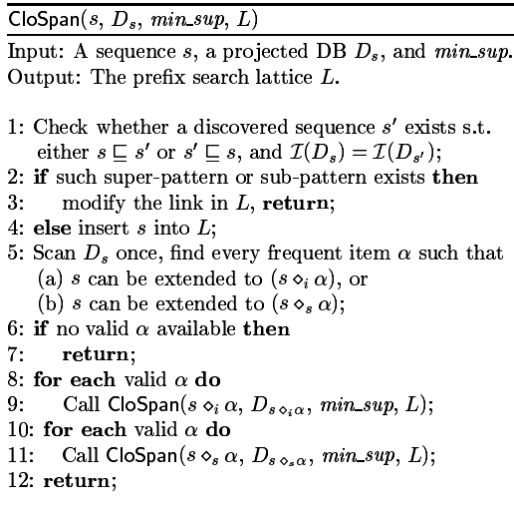
Figure 3. CloSpan Algorithm [5]
