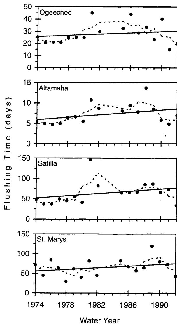
Figure 3. Flushing times in Georgia estuaries over 19 years. Dots are water-year averages, dashed lines are 3-year moving averages, and solid lines are linear regressions of 3-year moving averages.
