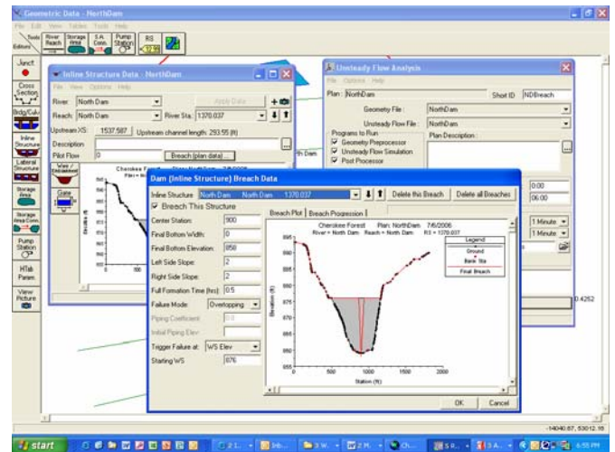
Figure 4 – Dam Breach Input
