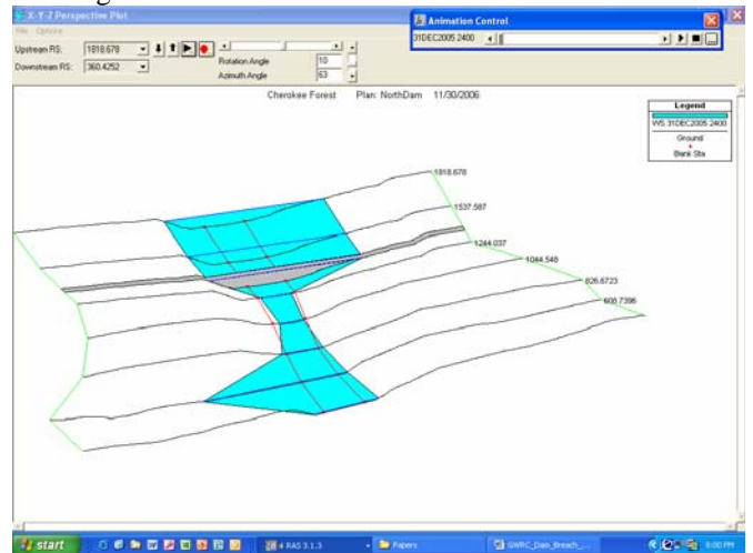
Figure 10 – Initial Conditions Three-Dimensional View
