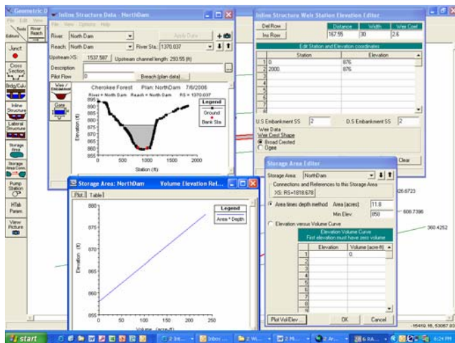
Figure 3 – In-line structure and storage area input screens
