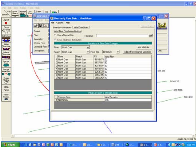
Figure 6 – Initial Flow Condition
