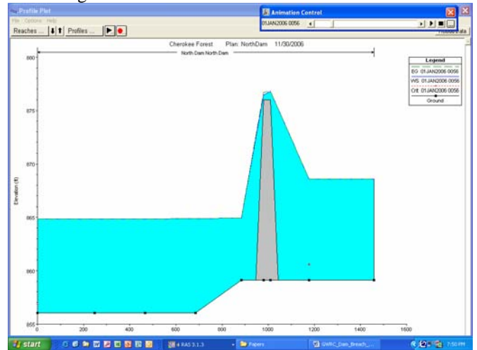
Figure 9 – Maximum Condition Results Profile
