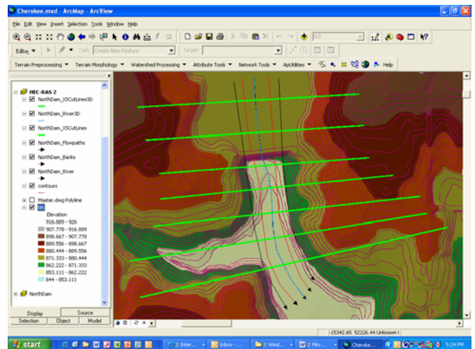
Figure 1 – HEC-GeoRAS GIS Platform
