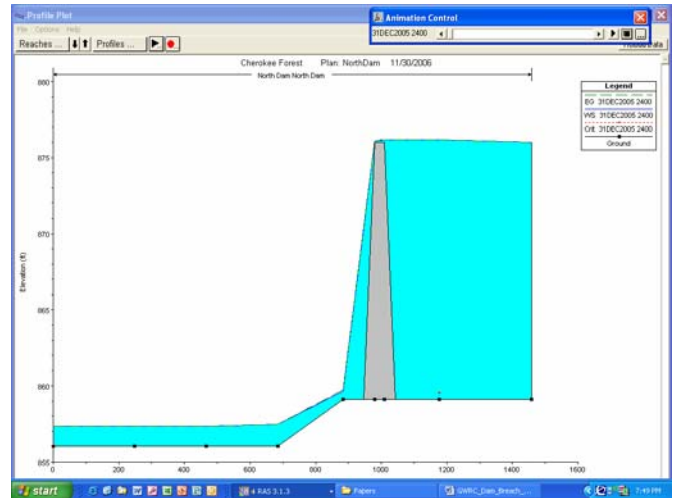
Figure 8 – Initial Condition Results Profile
