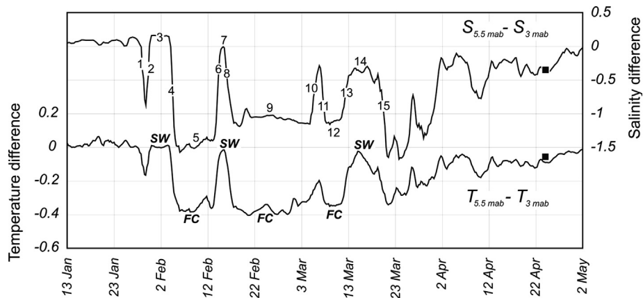
Fig. 3. The temporal evolution of 12-h running mean water temperature and salinity differences between 5.5 and 3 mab at Anabar mooring during 13 January–2 May 2008. Black squares indicate the T/S differences between 5.5 and 3 mab taken from a CTD cast at the pack ice 9 km north-west of Anabar mooring on 24 April.
