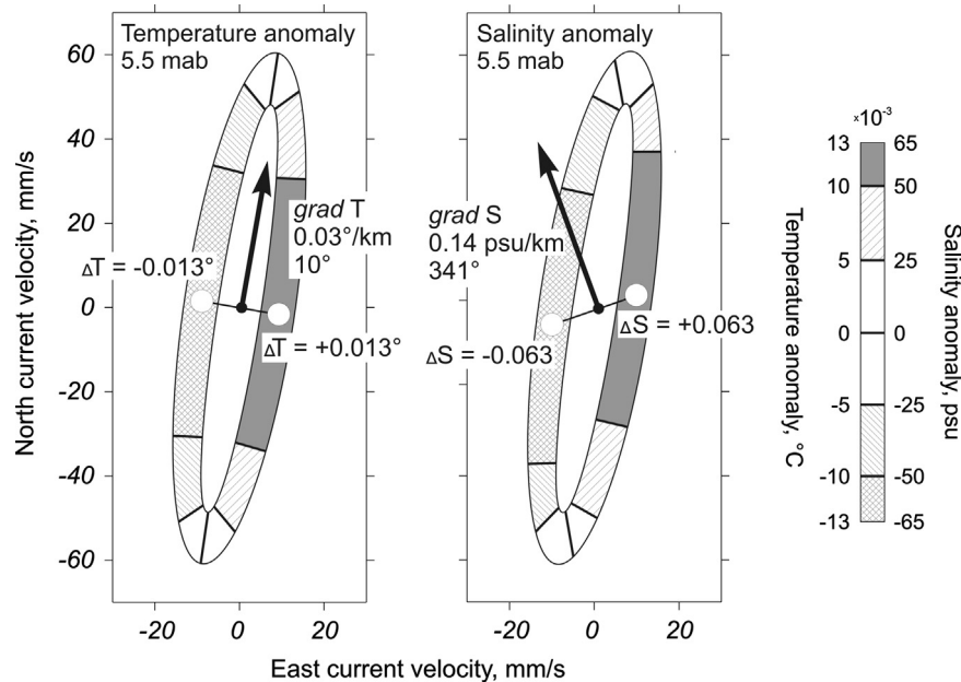
Fig. 5. The mean M_2 current ellipse and corresponding temperature and salinity oscillations at 5.5 mab during 29 January–21 March 2008. Arrows indicate the direction of cross-frontal temperature and salinity gradients.
