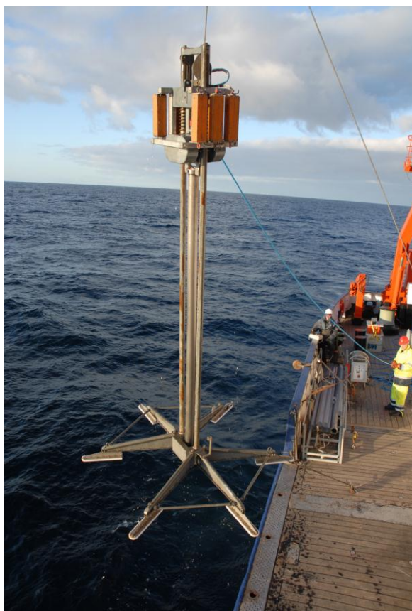
Fig. 4.4.1: Deployment of the vibrocorer.
