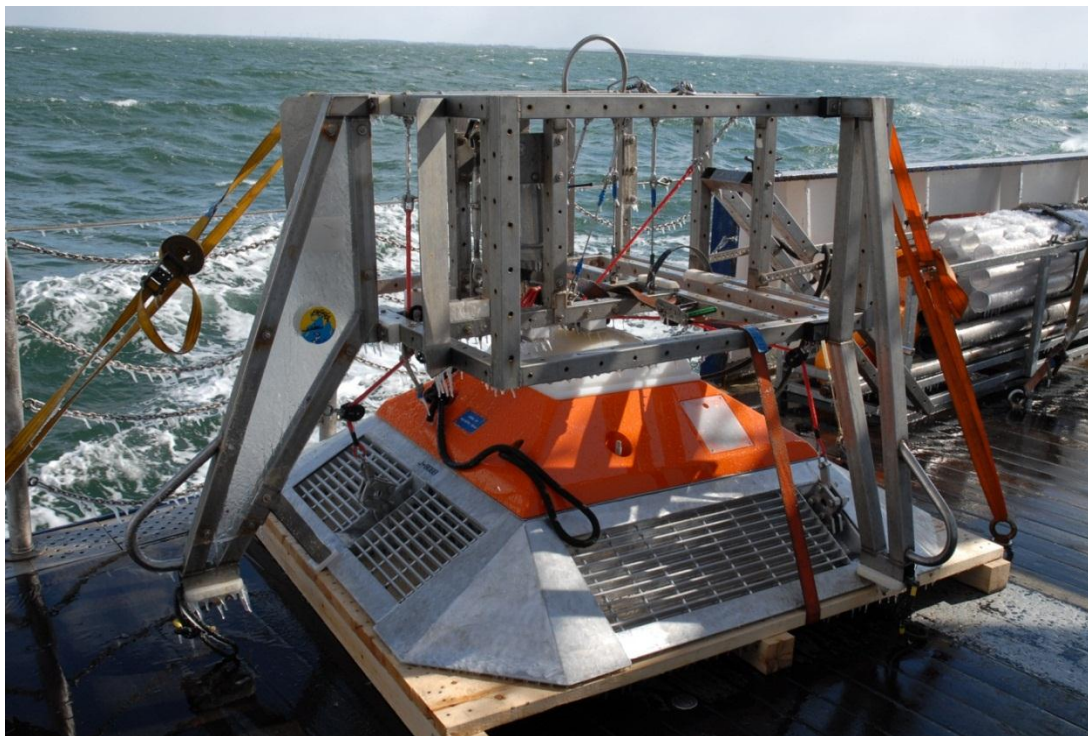
Fig. 2.1: Ice covered trawl-resistant lander with launcher on deck.
