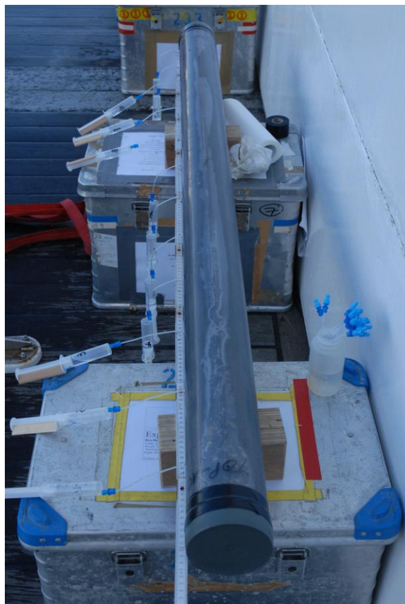
Fig. 4.4.2: Porewater extraction by rhizone sampling.
