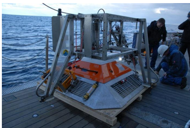
Fig. 4.3.1: Trawl resistant lander with launcher ready for deployment.
