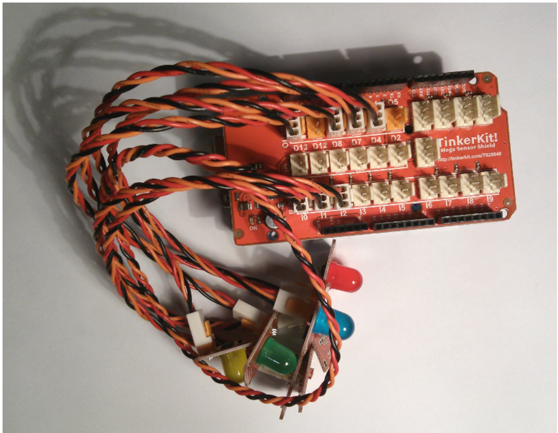
Figure 2.4: Complete Arduino Sensor Module
