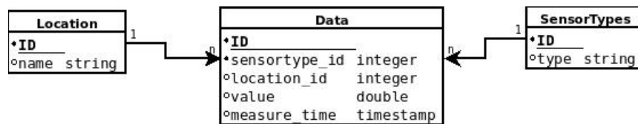
Figure 3.2: Server-side Data Model (2, p. 46)
