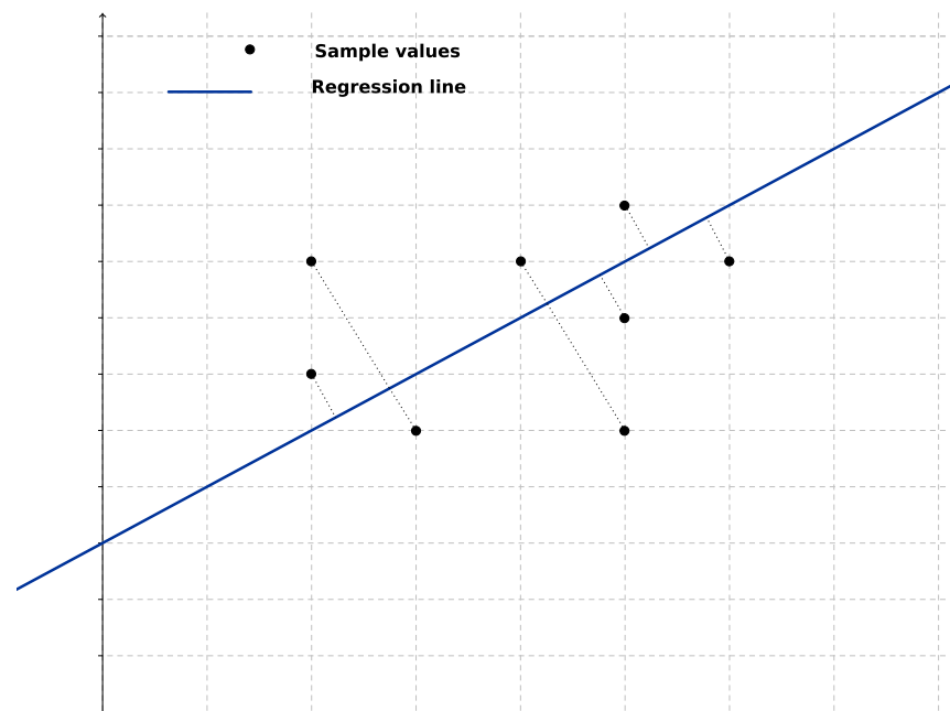
Figure 2.7: Least Squares Fitting Regression Line
