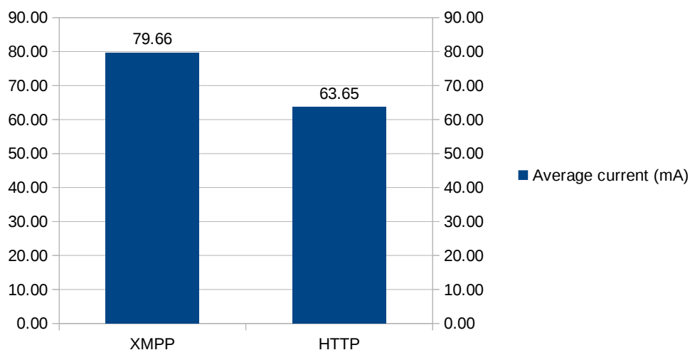
Figure 4.1: Power Consumption at 30 Second Interval
