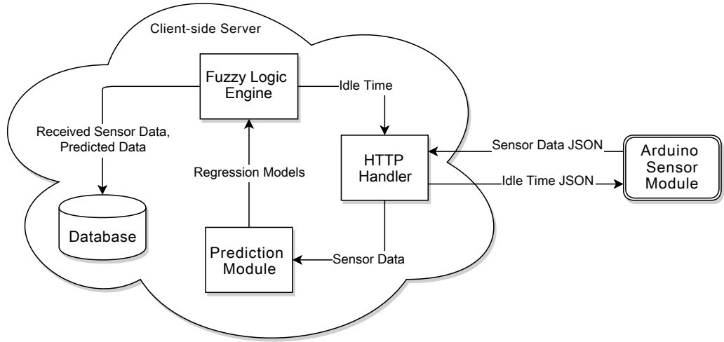
Figure 4.2: Final Solution Architecture
