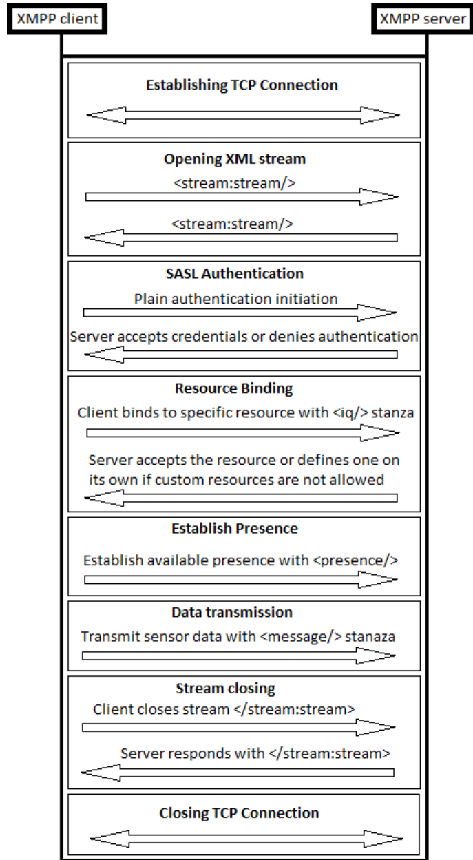
Figure 3.1: XMPP Session Lifecycle (2, p. 40)
