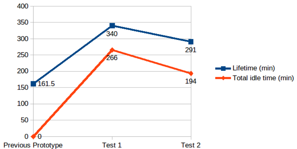
Figure 4.9: Battery Lifetime and Idle Time Comparison
