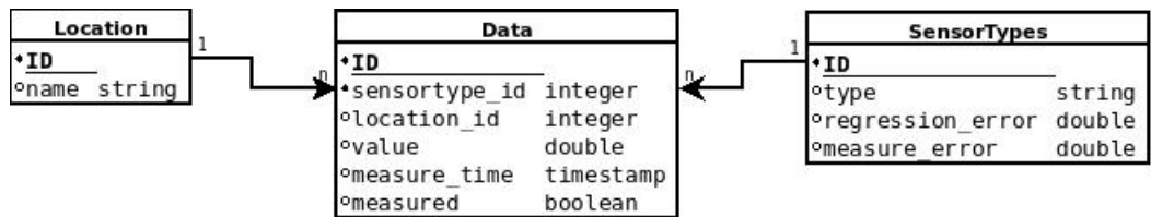
Figure 4.3: Updated Server-side Data Model
