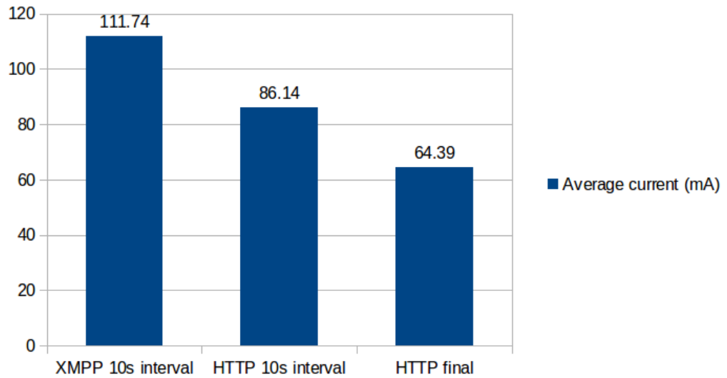
Figure 4.8: Current Measurements Comparison
