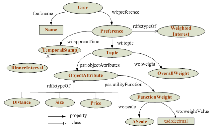
Figure 2. A User Preference Model
