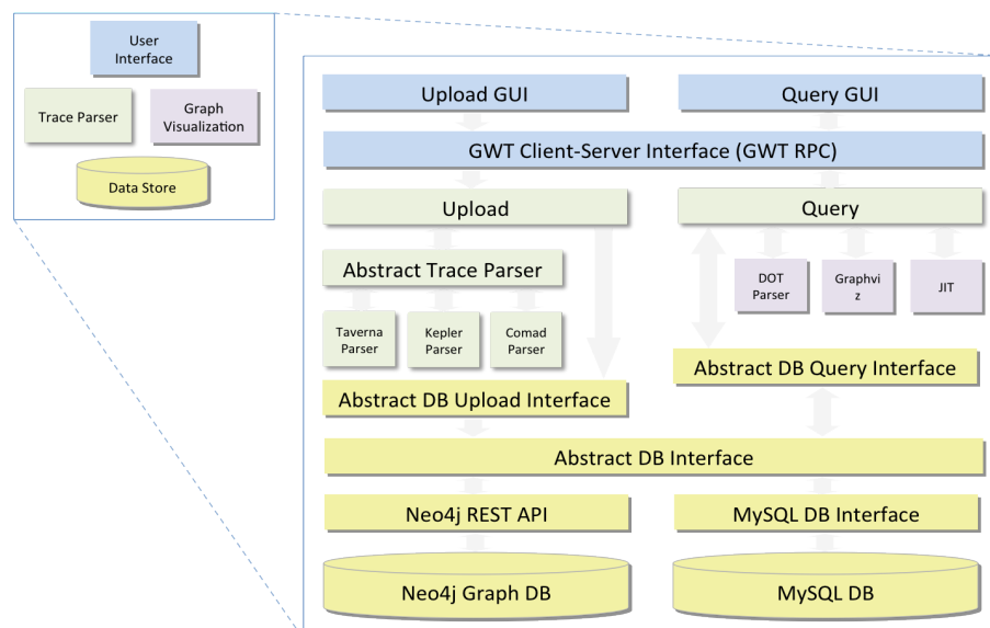
Figure 4. Golden-Trail architecture.
