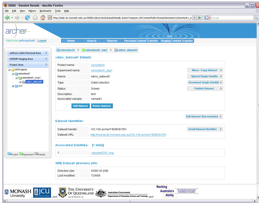
Figure 4. XDMS screenshot.
