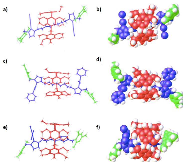
Figure 3. Views of the crystal structures of a, b) 2c ; c), d) 3c ; e), f) 3a . a), c) and e) ball-and-stick; b), d), f) space-filled representations. Blue = imidazolium/NHC rod, red = pillar[5]arene wheel, and green = mestyl stopper group.
