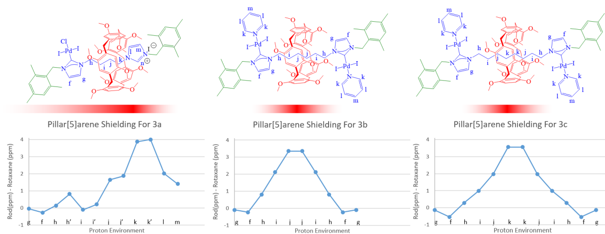
Figure 4. Calculated shielding effects [rod ^1\text{H} chemical shift (ppm) – rotaxane ^1\text{H} chemical shift (ppm)] for [2]rotaxanes 3a-c indicating the favoured residency of the pillar[5]arene on the rod.
