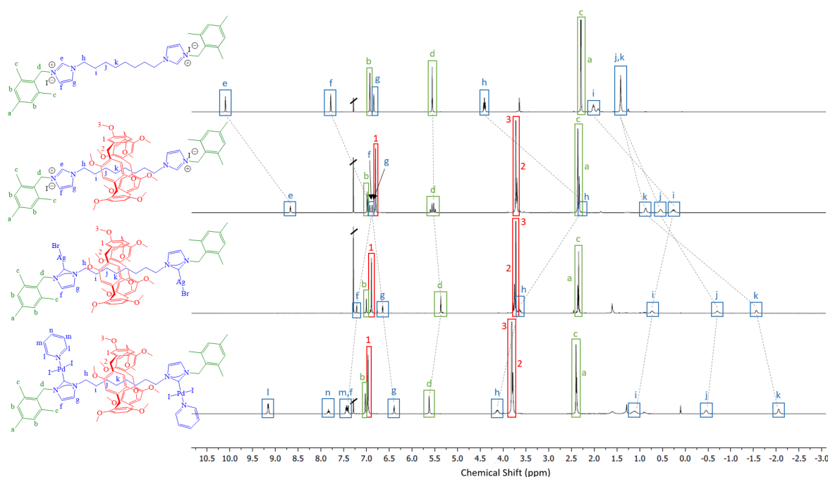
Figure 1. 1 H NMR spectra (400 MHz, CDCl 3 , 298 K) schematic showing the NMR shifts of 1c due to the confinement of the pillar[5]arene by the coordination of Ag(I) 2c or Pd(II) 3c . Bis-imidazolium rod 4c (top) is included for comparison.
