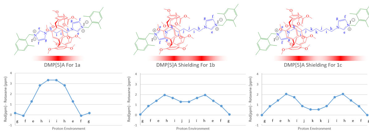
Figure 2. Calculated shielding effects [rod ^1\text{H} chemical shift (ppm) – rotaxane ^1\text{H} chemical shift (ppm)] for [2]rotaxanes 1a-c indicating the favoured residency of the pillar[5]arene on the rod.
