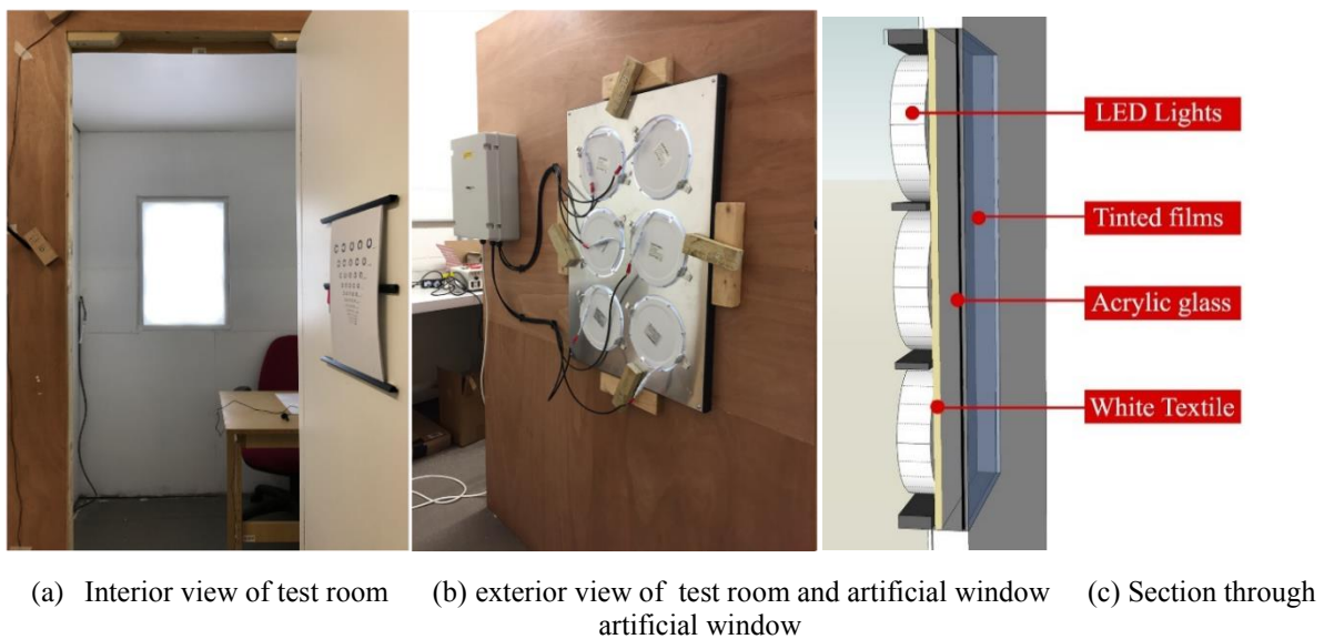
Figure 2: The configuration of the designed artificial window
