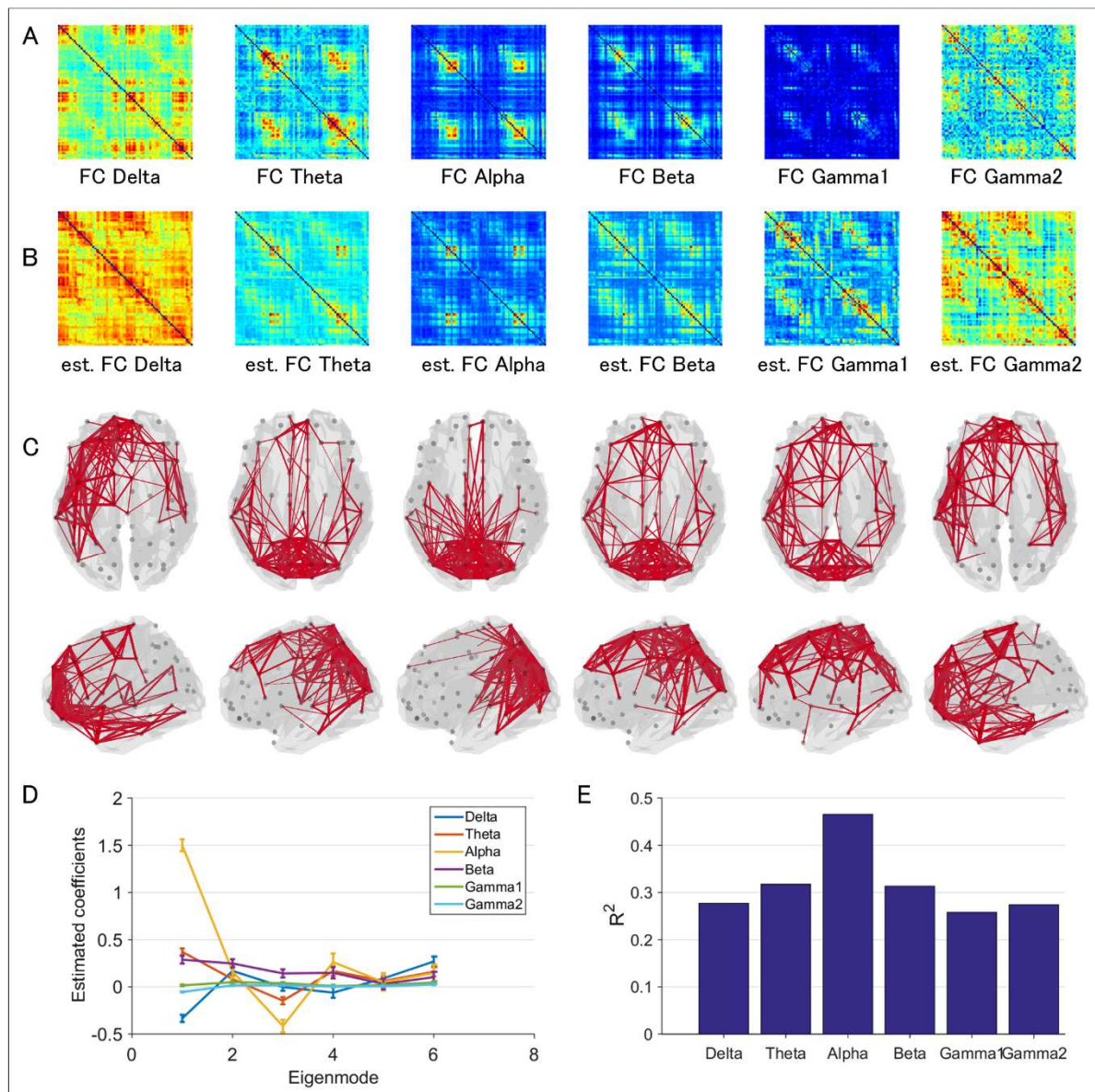
Figure 2 Prediction of frequency band specific networks based on the eigenmodes: (A) Frequency band specific functional connectivity matrices based on AEC and MEG data. (B) Predicted functional connectivity matrices based on a linear weighted sum of the first six eigenmodes of the structural connectome. Colours in A and B correspond to connectivity strength (C) Predicted functional connections using a linear weighted sum of the structural eigenmodes, illustrated in glass brain plots. (D) shows the estimated coefficients for the first six eigenmodes, i.e. it shows how much each eigenmode contributes to a frequency band specific prediction. Error bars correspond to the confidence intervals of the estimated coefficients. (E) shows how much of the variance ( R^2 ) of the empirical functional connectivity matrices can be explained by a linear combination of the eigenmodes for each frequency band separately.
