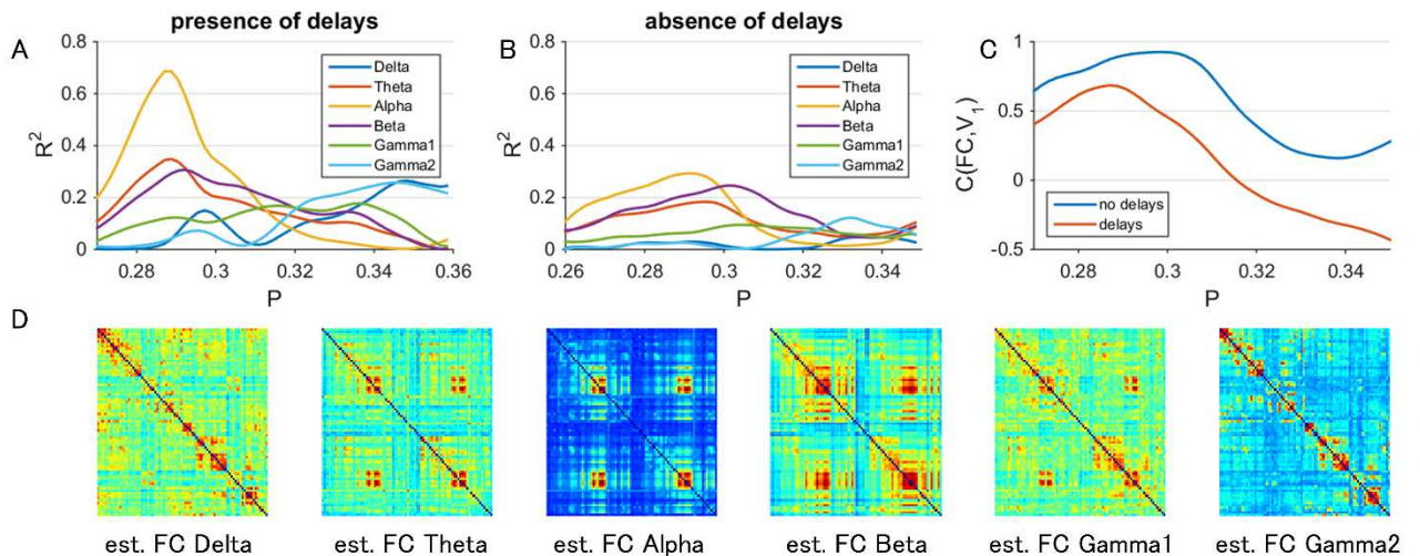
Figure 5 Simulations of a network of neural masses in the presence and absence of delays: (A) shows the goodness of fit in terms of the R^2 between simulated functional connectivity matrices and MEG connectivity matrices for different values for P , for different frequency bands in the presence of delays. (B) shows the equivalent of (A) in the absence of delays. (C) shows the correlation between simulated functional connectivity matrices and the first eigenmode of the structural connectome in the absence (blue) and presence (red) of delays for various values for P . (D) shows the best fits for the model output with empirical MEG data. The matrices correspond to values for P for which the curves in (A) are maximal.
