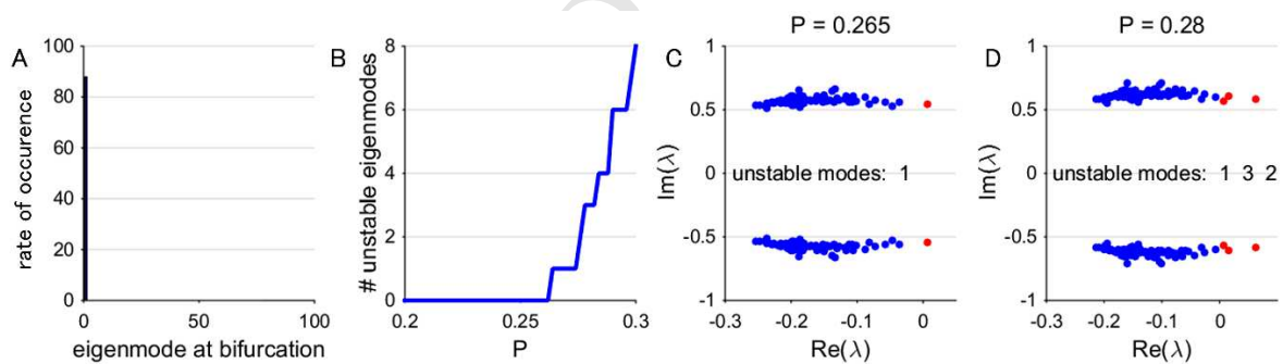
Figure 3 Linear stability analysis of a network of neural mass models in the absence of delays: (A) the eigenmodes that become unstable at the bifurcation. It is always the first eigenmode in the absence of delays that crosses the bifurcation and thus loses stability. This bifurcation occurs for P = 0.26 (B), i.e. this is the value for P when an eigenmode loses stability. By increasing P further, other eigenmodes also lose their stability (B). (E) shows the eigenspectrum of the system right after the bifurcation in the absence of delays. Here only the first eigenmode loses stability (complex conjugate pair) (F) shows an example of the spectrum in the absence of delays further away from the bifurcation when multiple eigenmodes lose their stability. Blue dots in (C-D) correspond to \lambda that are stable, while red dots correspond to \lambda that are unstable and thus excited.
