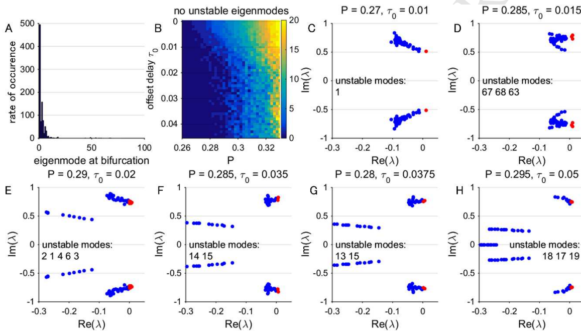
Figure 4 Linear stability analysis of a network of neural mass models in the presence of delays: (A) the eigenmodes that lose their stability at the bifurcation. Delays allow other eigenmodes than the first one to lose their stability at the bifurcation. A bifurcation occurs in (B) when the real part of the system eigenvalues cross the imaginary axis in the complex plane. Both P and \tau_0 are tuned in (B). (C-F) show different eigenspectra for different values for the offset delay ( \tau_0 ), and demonstrate how various other eigenmodes can be excited at the bifurcation. It also demonstrates how the presence of delays allows to excite eigenmodes nearly simultaneously. (E) shows the eigenspectra where the correct eigenmodes (Figure 2D) are excited nearly simultaneously. Blue dots in (C-H) correspond to \lambda that are stable, while red dots correspond to \lambda that are unstable and thus excited.
