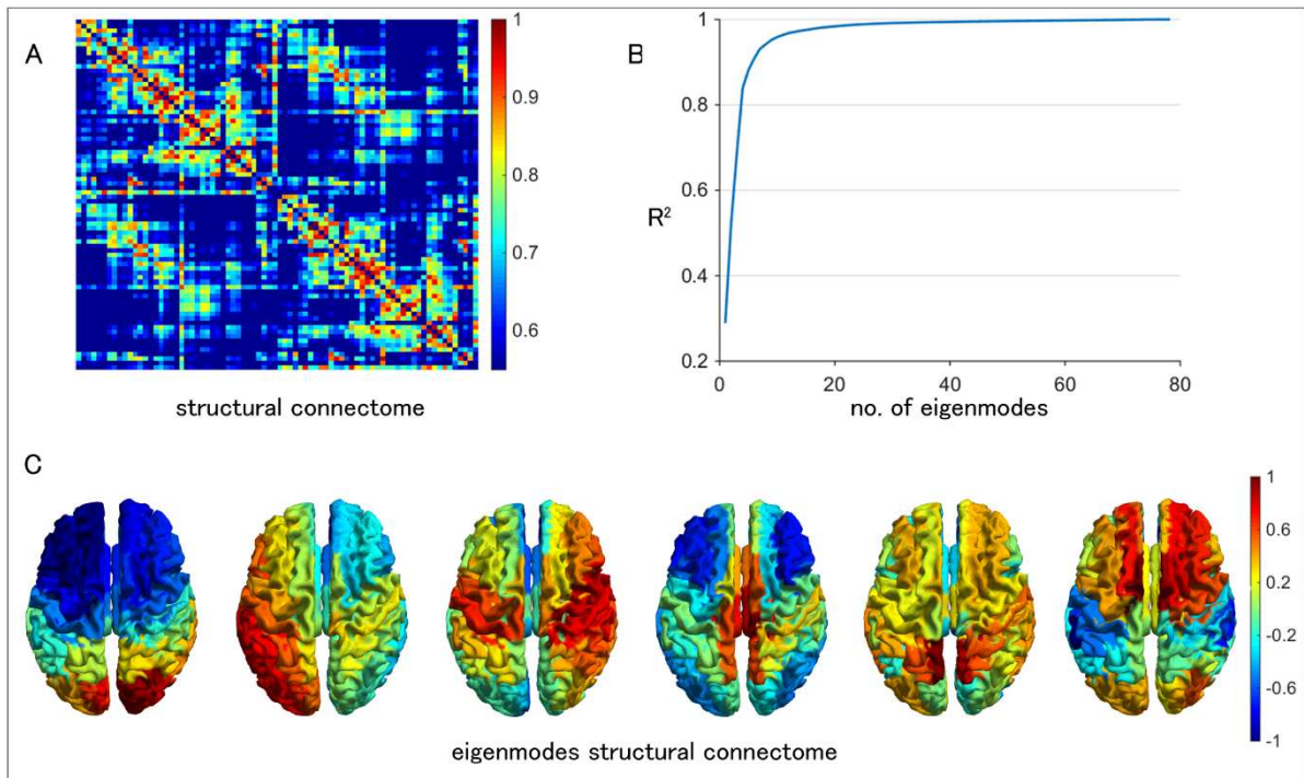
Figure 1 Structural connectome: (A) The weighted adjacency matrix of the structural connectome with a link density of 0.37. (B) The variance of structural connectome ( R^2 ) explained by the first n structural eigenmodes. The variance explained for n number of eigenmodes in the graph corresponds to the set from the first eigenmode on to the n^{\text{th}} eigenmode. (C) As an illustration, the first six eigenvectors of the structural connectome are depicted from left to right in an ascending order.
