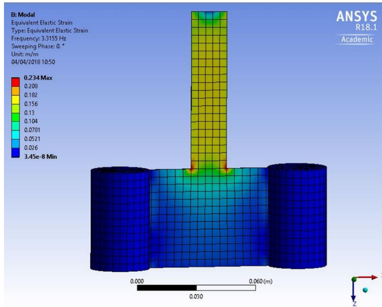
Figure 8. The strain distribution calculated by the FEM
