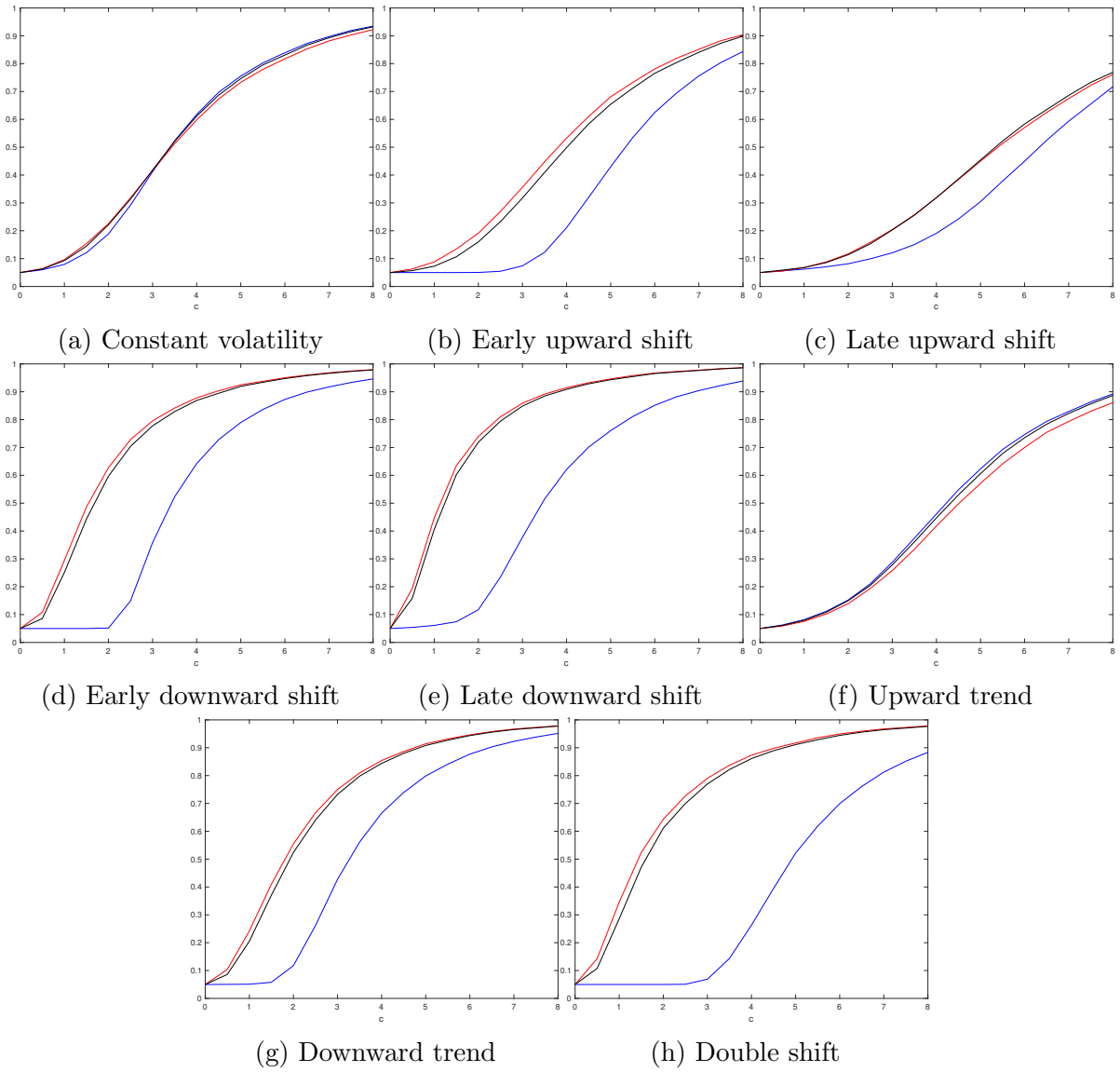
Figure 1: Limiting local power curves, \tau^* = 0.6 , \text{supDF} : —, \text{supBZ} : —, \mathcal{U} : —.
