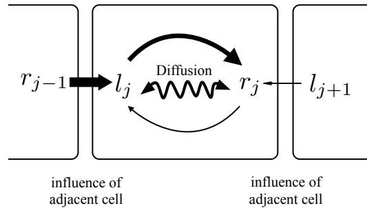
Figure 10: Schematic representation of the mechanism of the conservative model. A conserved PCP activity within each cell is redistributed in response to juxtacrine intercellular signalling and intracellular diffusion.
