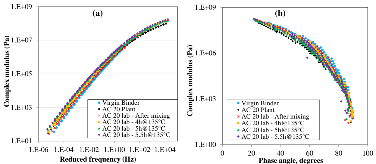
Figure 2. (a) Complex Modulus Master Curves (b) Black Space Diagrams for Virgin 40/60 Pen Asphalt and Binder Recovered from Plant and Laboratory Produced Mixtures
