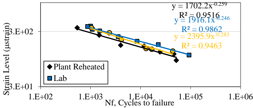
Figure 5. Strain vs N_f Plot from ITFT for Different Mixtures
