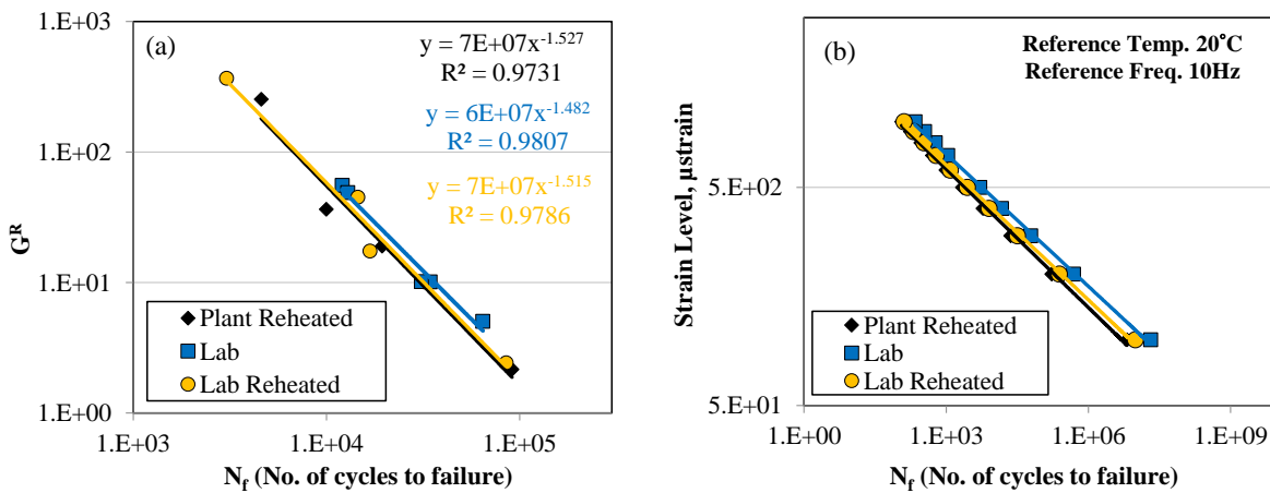
Figure 6. (a) G^R vs N_f (b) Predicted Strain vs N_f Plot for Different Mixtures
