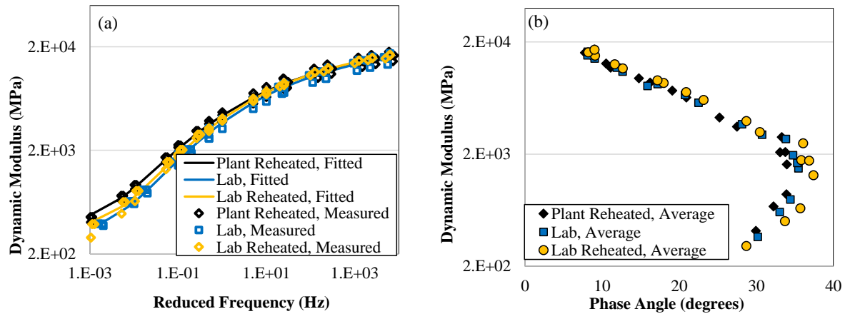
Figure 4. (a) Dynamic Modulus Master Curves (b) Black Space Diagrams for Different Mixtures
