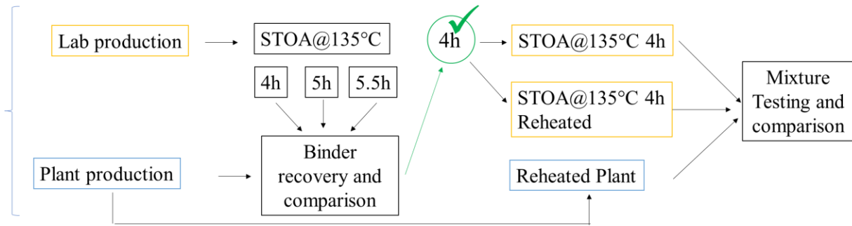
Figure 1. Short-term Aging Approach for Binders and Mixtures
