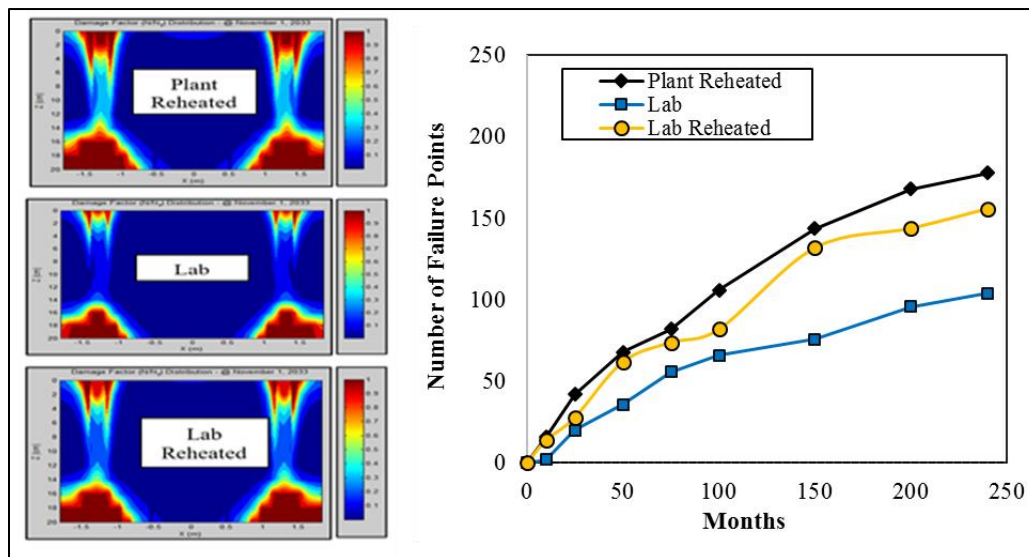
Figure 7. Number of Failure Points Over Time Due to Total Cracking
