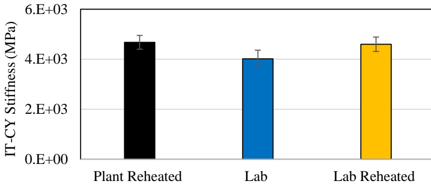
Figure 3. IT-CY Stiffness Results of Plant and Laboratory Produced Mixtures
