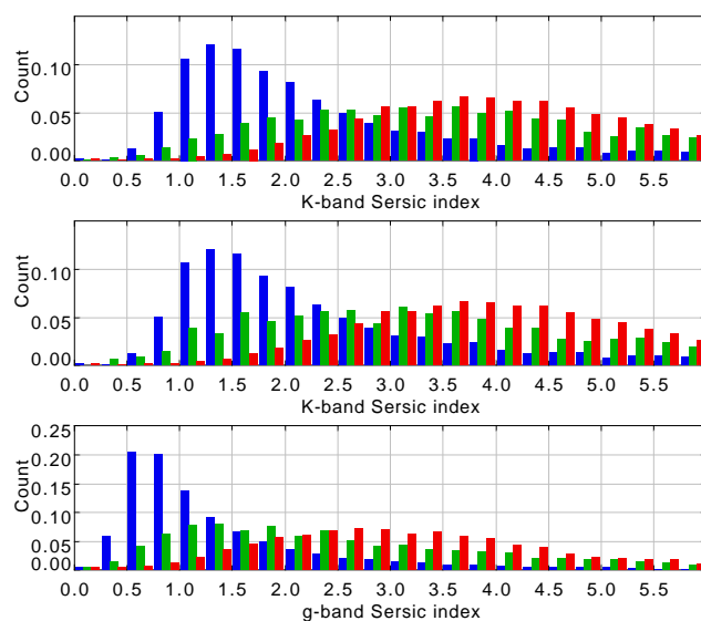
Figure 6. Top: Normalised histogram of K -band Sérsic index distribution for the red, green and blue subsamples, clearly demonstrating the significant difference of the distribution for the blue galaxies and the similarity for those of the green and red galaxies. Less than 10 per cent of the green galaxies need to be re-distributed in Sérsic index for the red and green distributions to be statistically indistinguishable. Middle: The same plot, but this time only including the bluest third of the green sample. These have a mean u^* - r^* \sim 1.35 , only 0.15 magnitudes redder than the mean colour of the blue subsample. Despite this small difference in colour, the green distribution is still far closer to that of the red subsample (which has a mean u^* - r^* \sim 1.9 ) than that of the blue, with only a \sim 5 per cent increase in the fraction of sources with n < 2.5 in comparison to the complete green sample. Bottom: The same as the top histogram, but this time measuring the distribution of g -band Sérsic indices. In this case the complete green subsample has a Sérsic distribution intermediate between those of the blue and red subsamples, as expected from previous work. The difference in g - and K -band measurements are caused by the near-IR surface brightness profile being a better tracer of the underlying stellar mass distribution than the optical surface brightness profile and thus demonstrating that the mass profiles for green and red galaxies are extremely similar.
